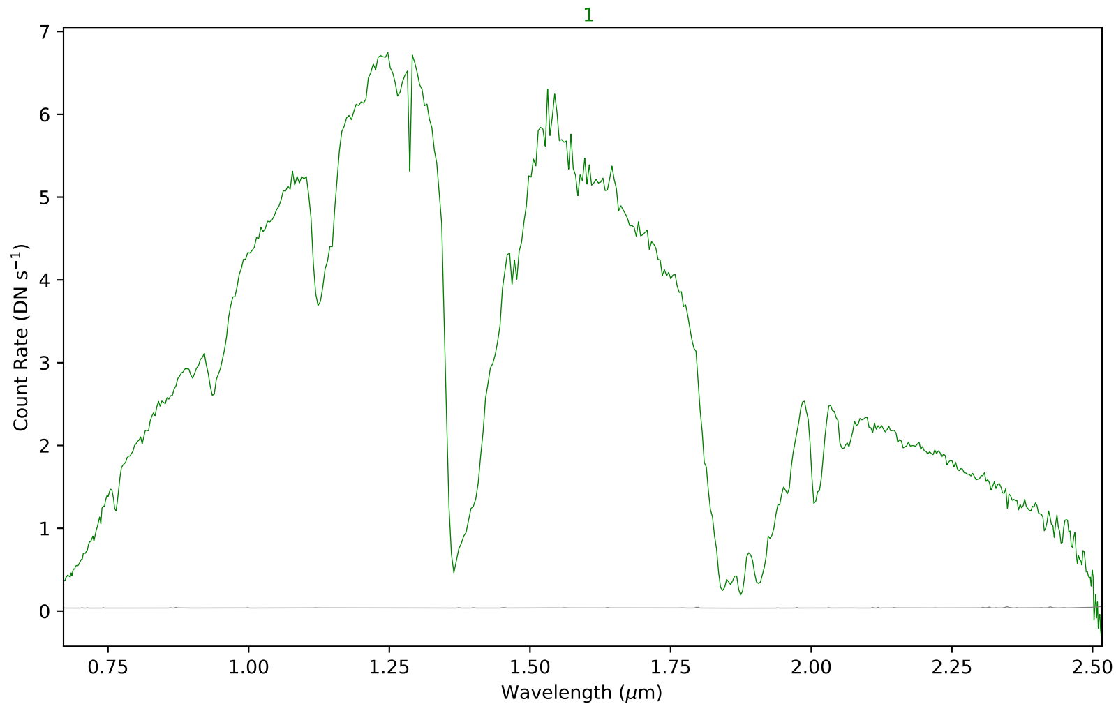
combspec777-788.fits - Aperture 1
