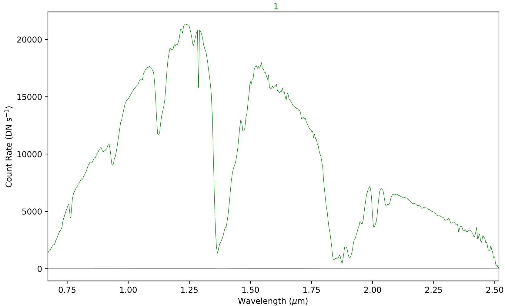
combspec813-818.fits - Aperture 1
