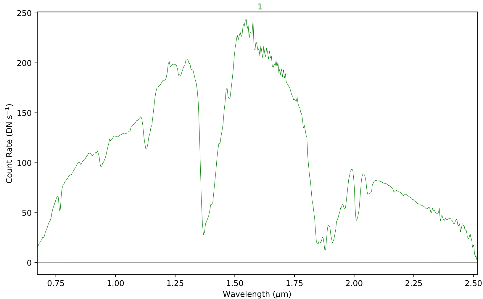
combspec131-142.fits - Aperture 1
