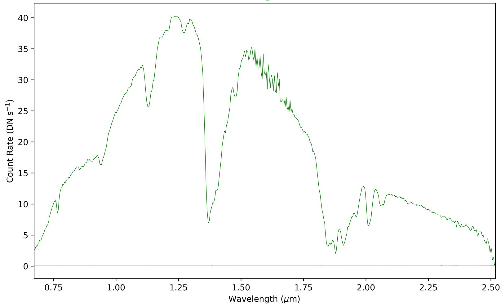
combspec167-174.fits - Aperture 1
