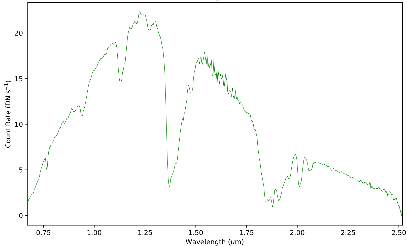
combspec175-186.fits - Aperture 1
