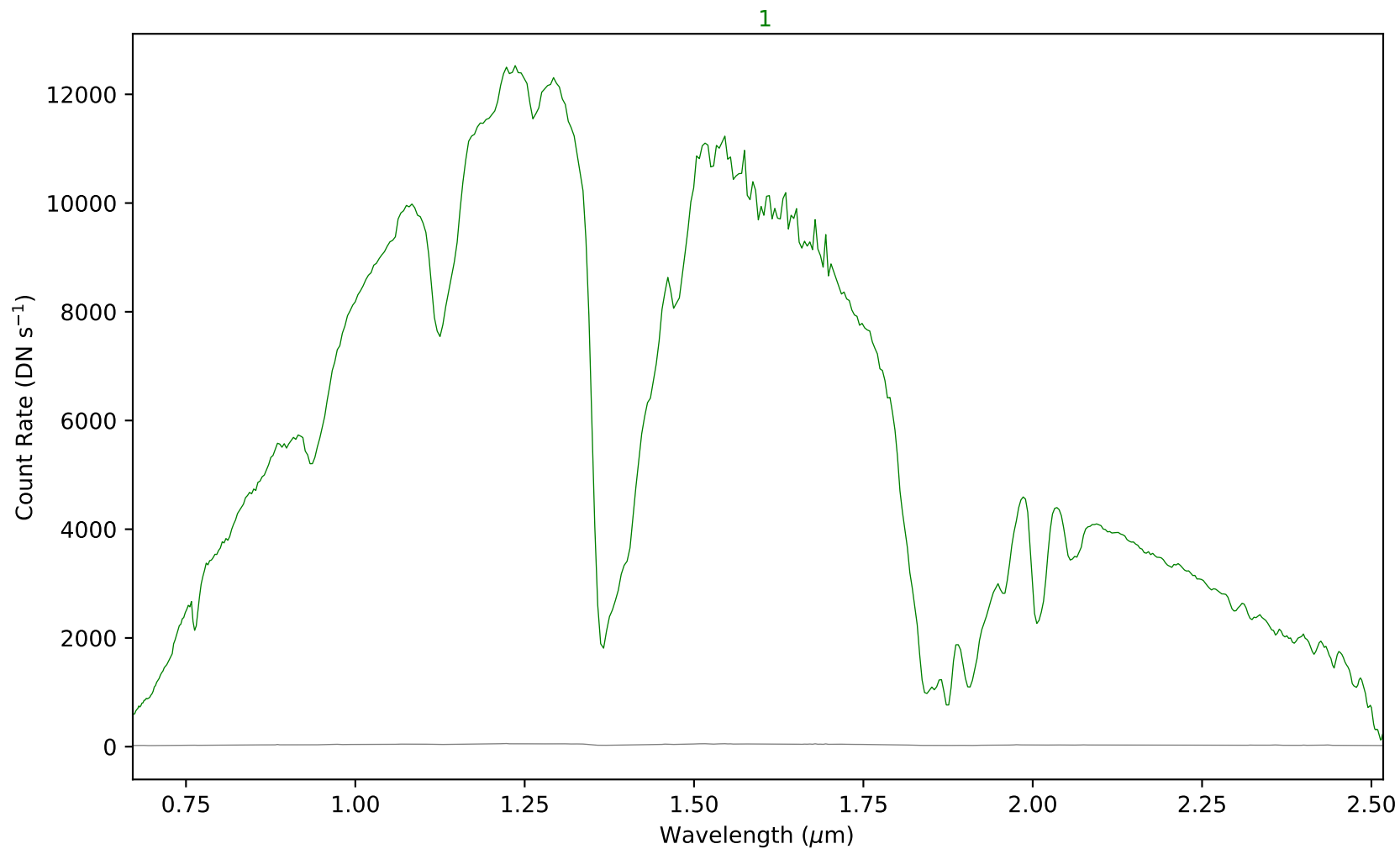
combspec205-408.fits - Aperture 1
