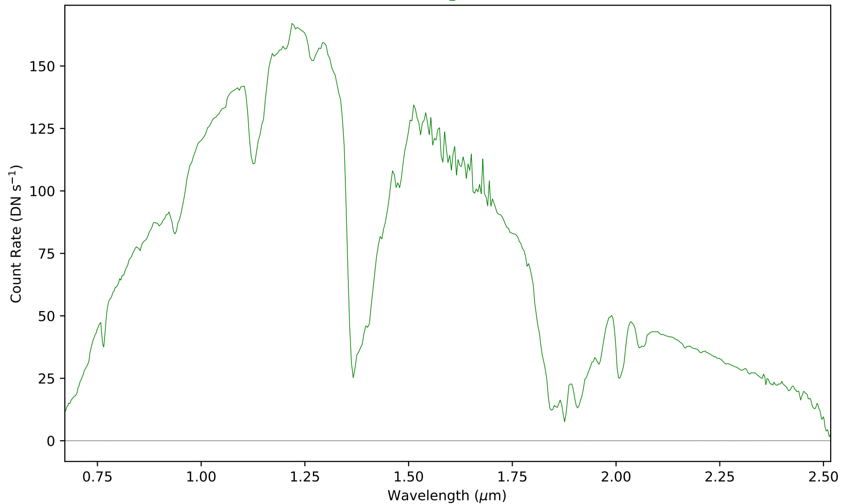
combspec223-246.fits - Aperture 1
