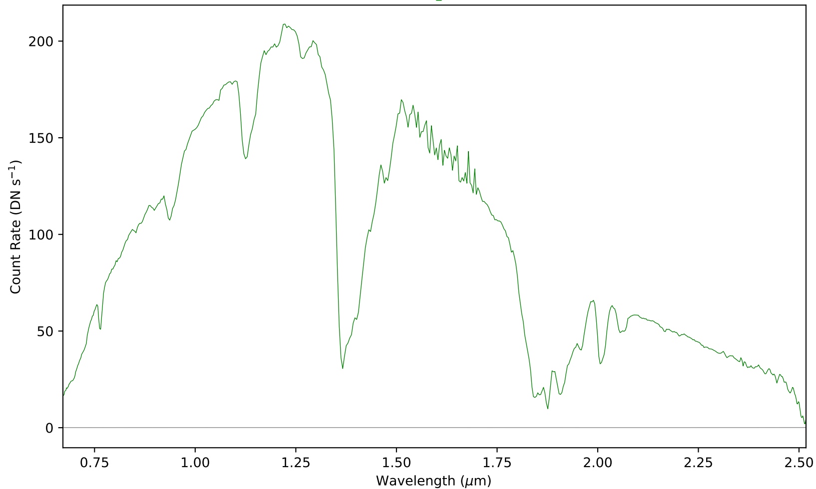
combspec247-258.fits - Aperture 1
