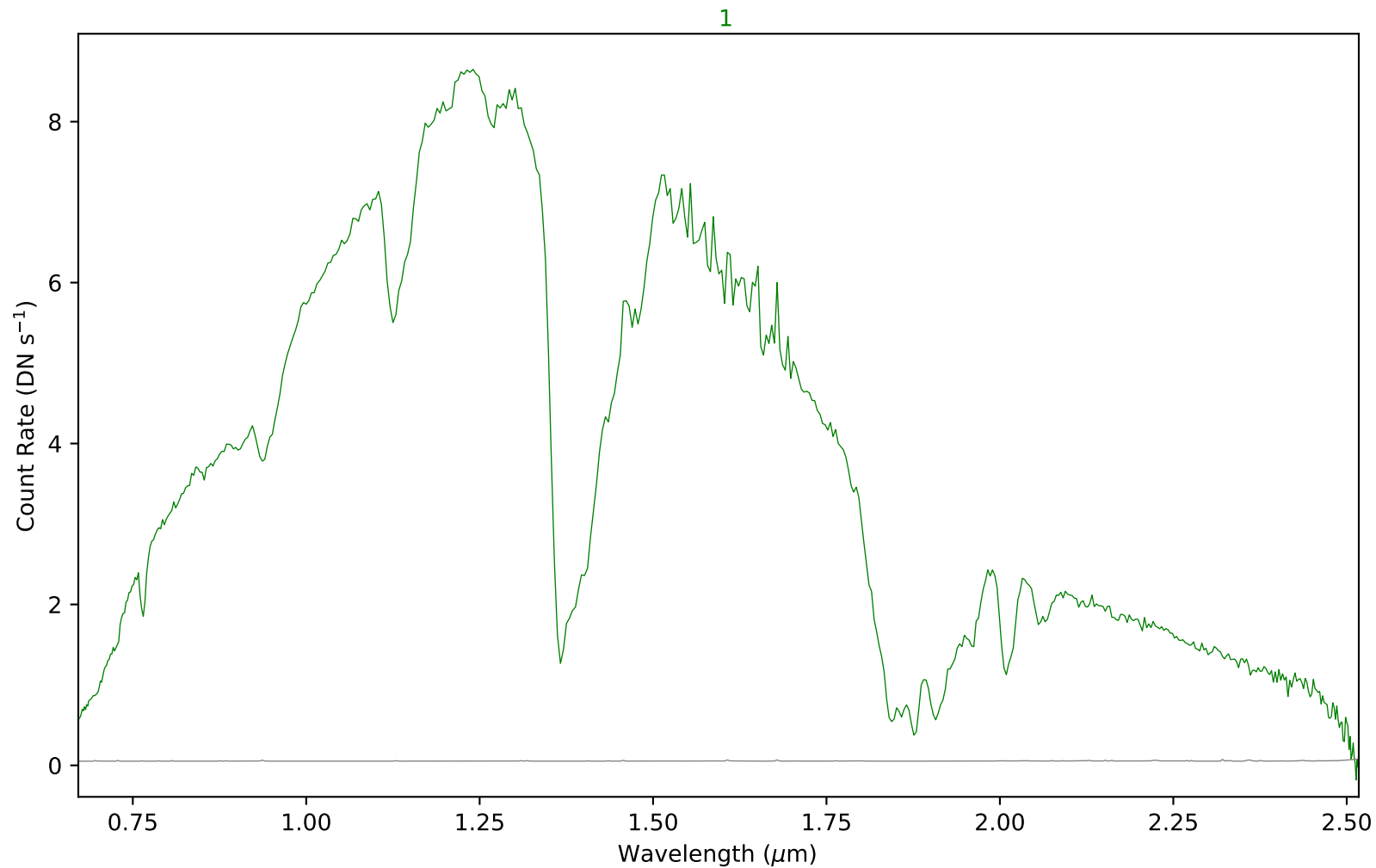
combspec283-292.fits - Aperture 1
