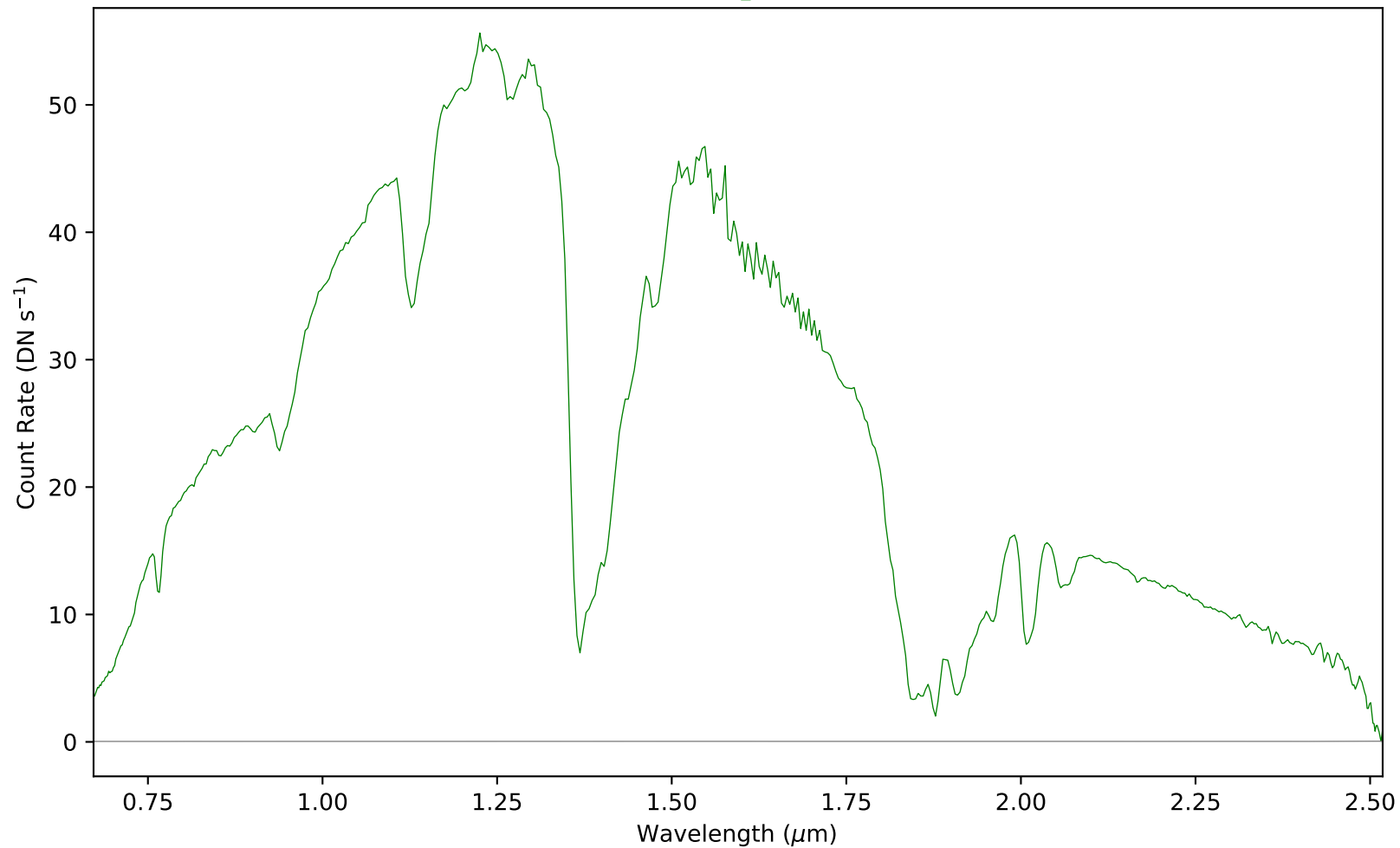
combspec31-44.fits - Aperture 1
