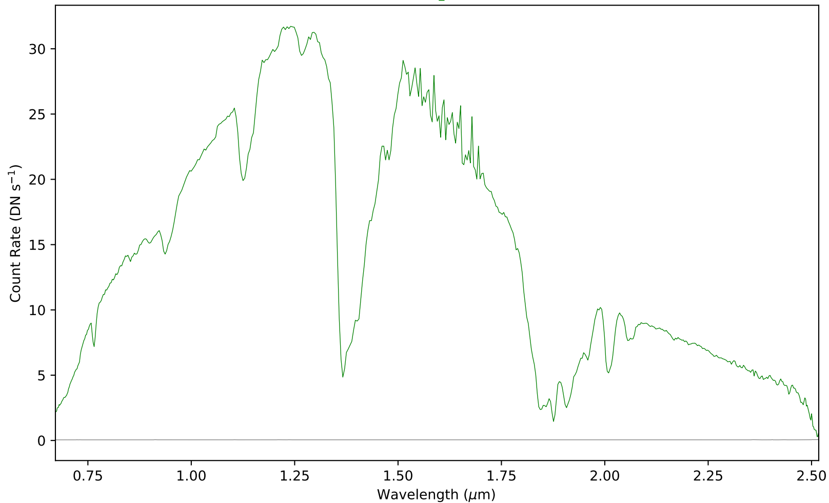
combspec335-344.fits - Aperture 1
