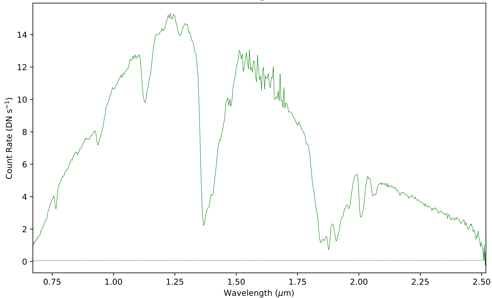
combspec345-352.fits - Aperture 1
