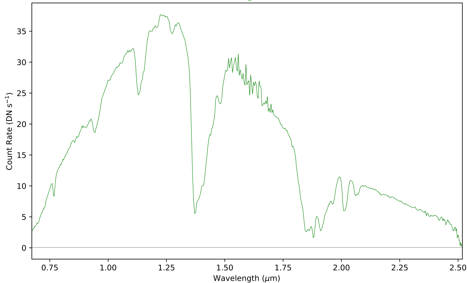
combspec353-360.fits - Aperture 1
