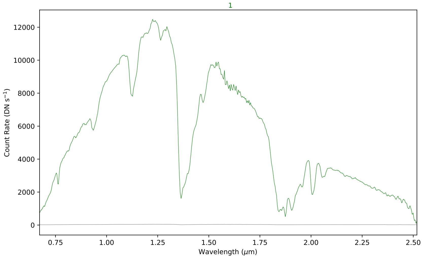
combspec45-154.fits - Aperture 1
