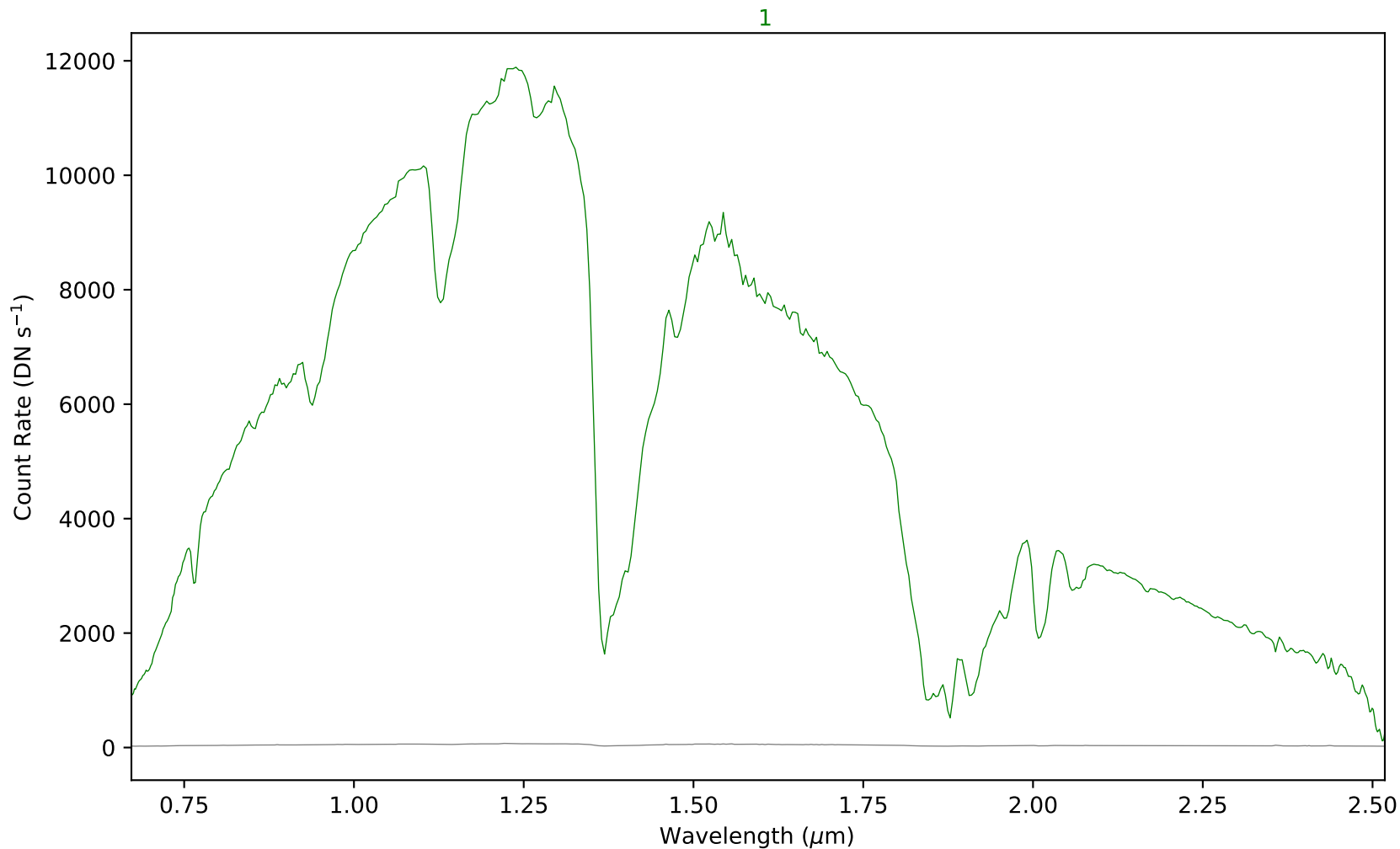
combspec463-524.fits - Aperture 1
