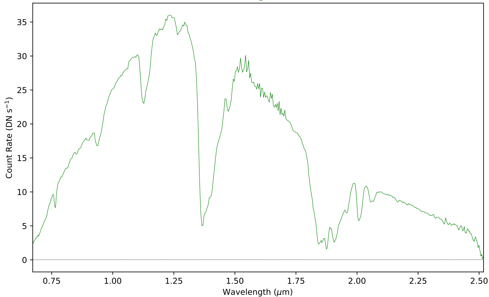
combspec475-492.fits - Aperture 1
