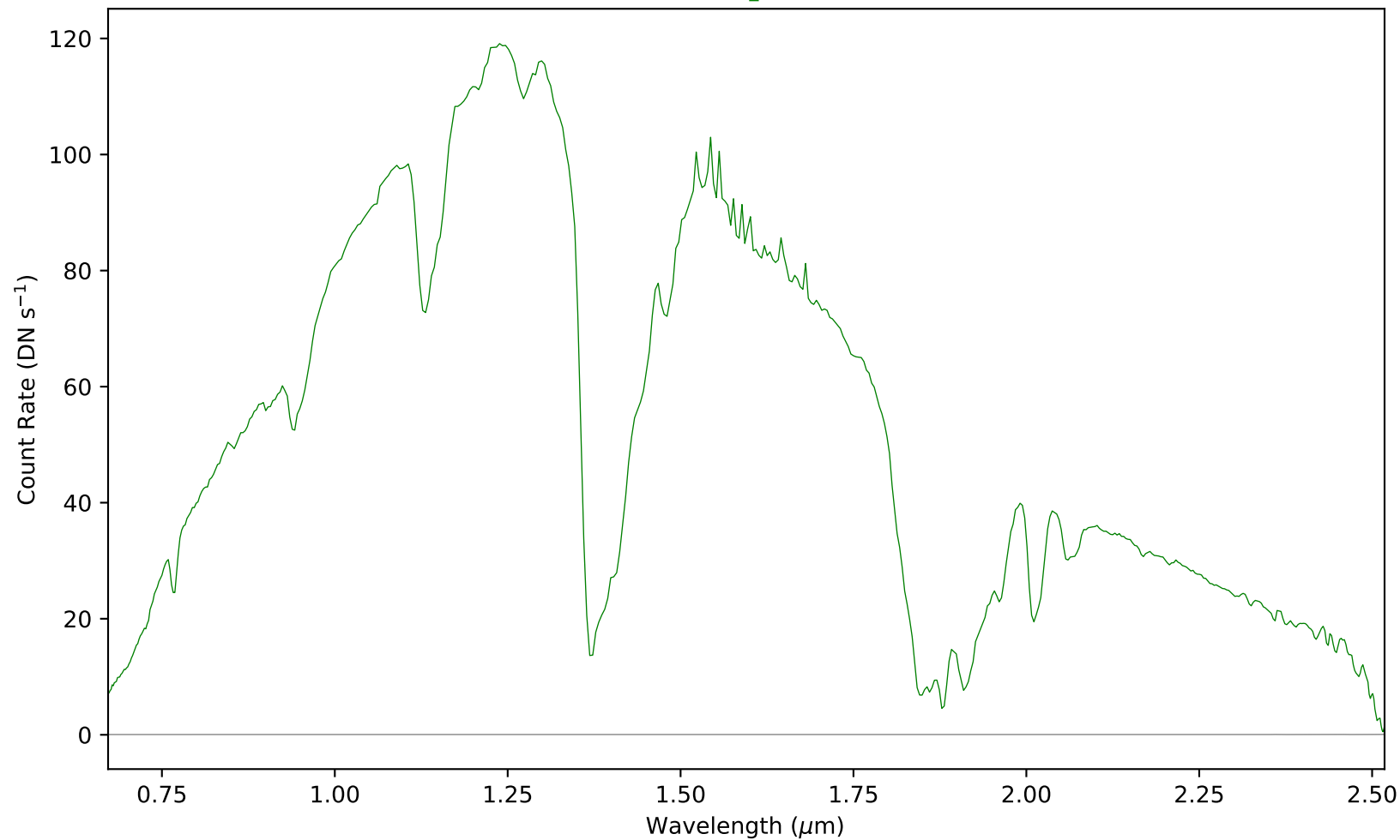
combspec531-540.fits - Aperture 1
