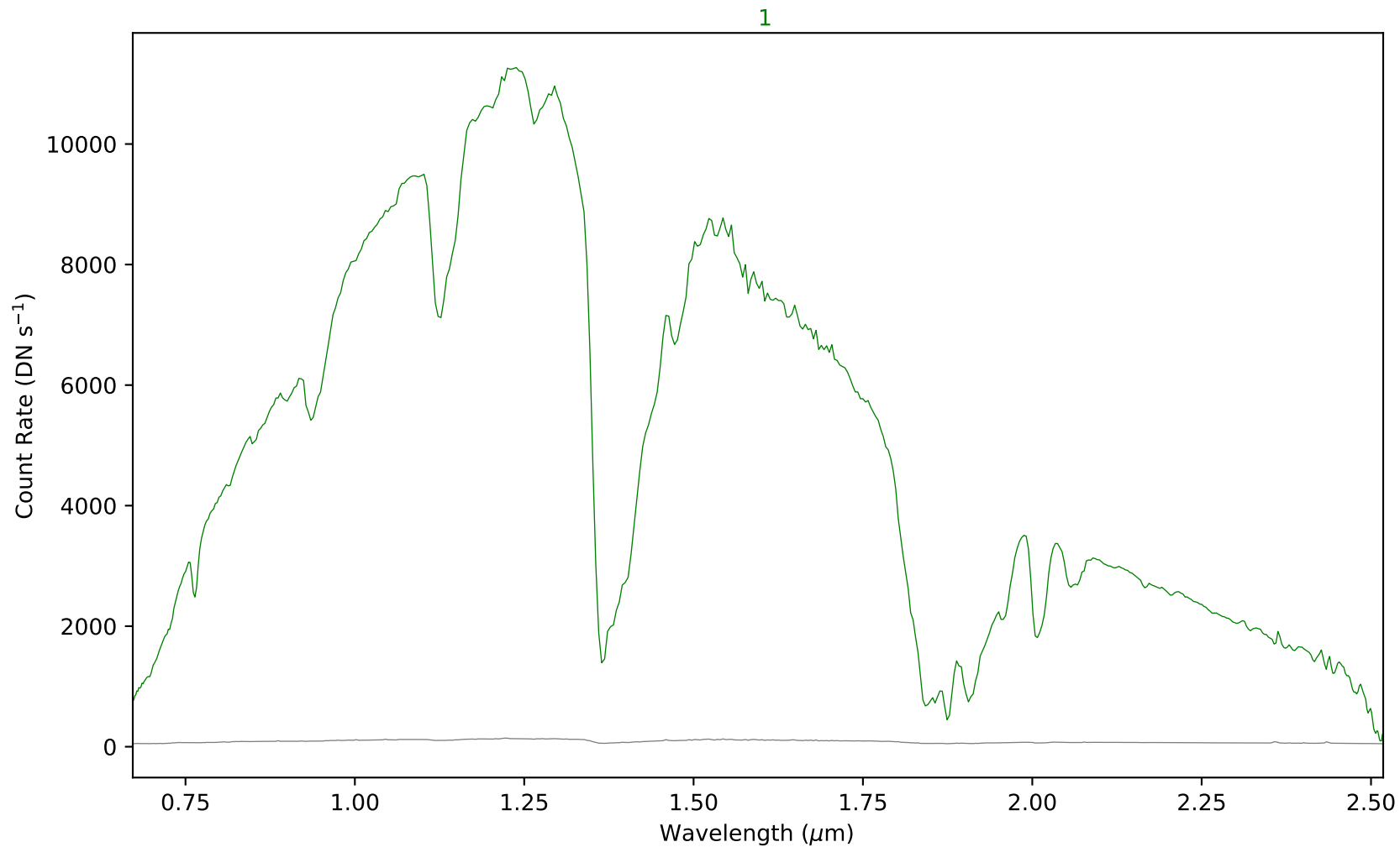
combspec553-564.fits - Aperture 1
