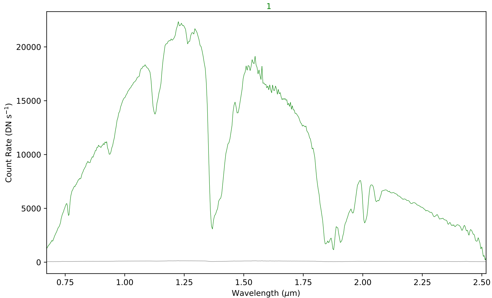
combspec57-198.fits - Aperture 1
