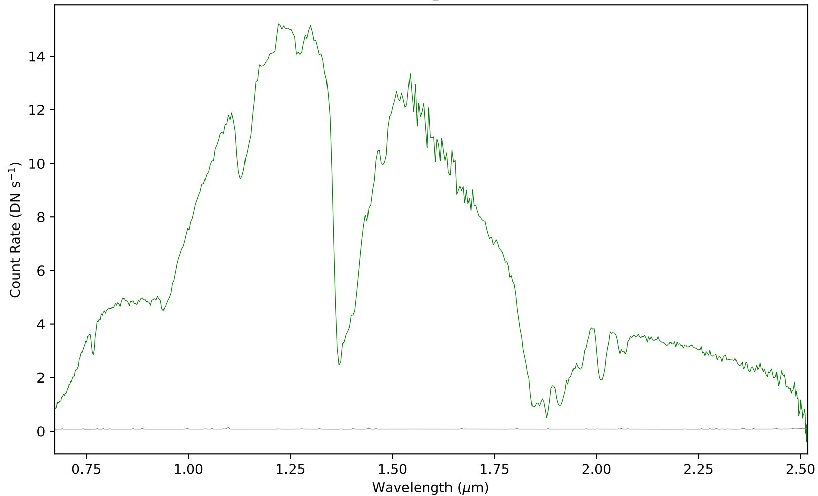
combspec69-74.fits - Aperture 1
