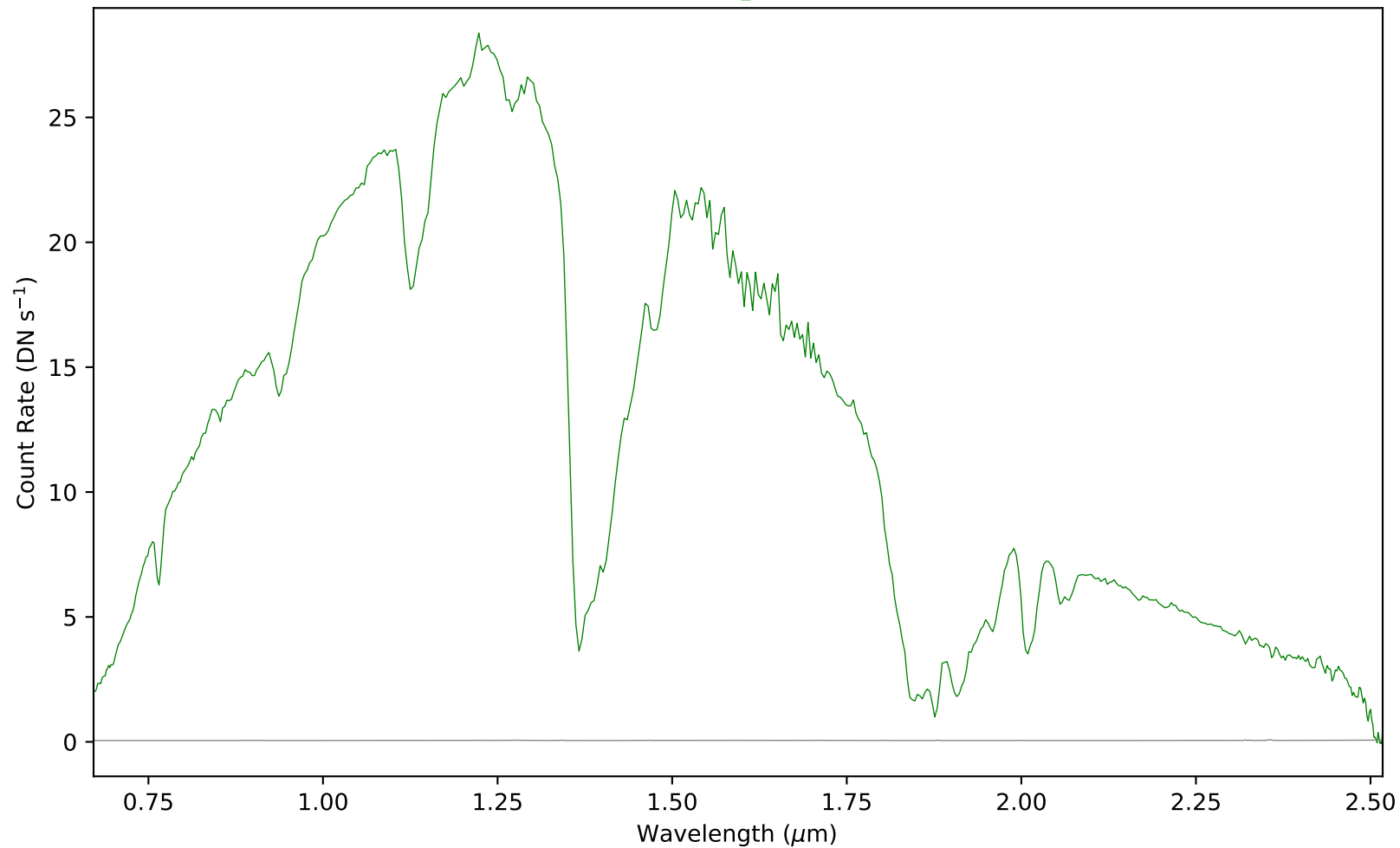
combspec1-10.fits - Aperture 1
