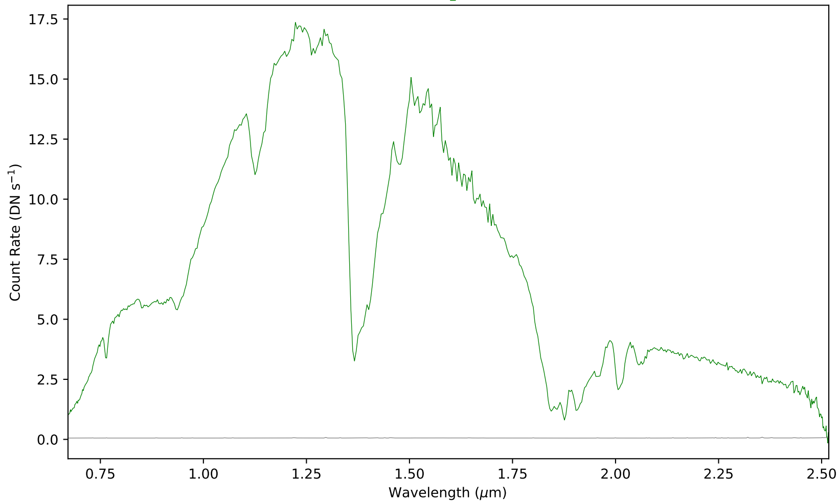
combspec146-181.fits - Aperture 1
