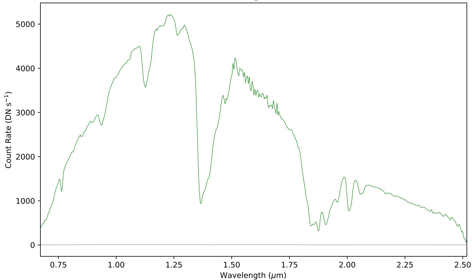
combspec192-369.fits - Aperture 1
