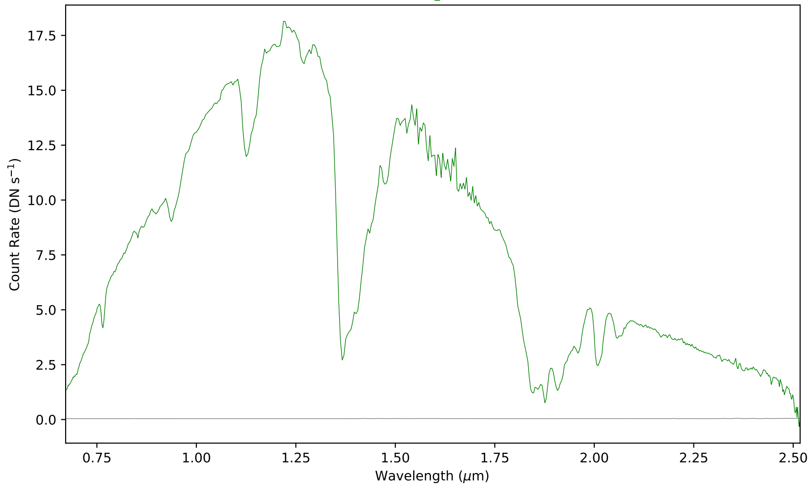
combspec212-223.fits - Aperture 1
