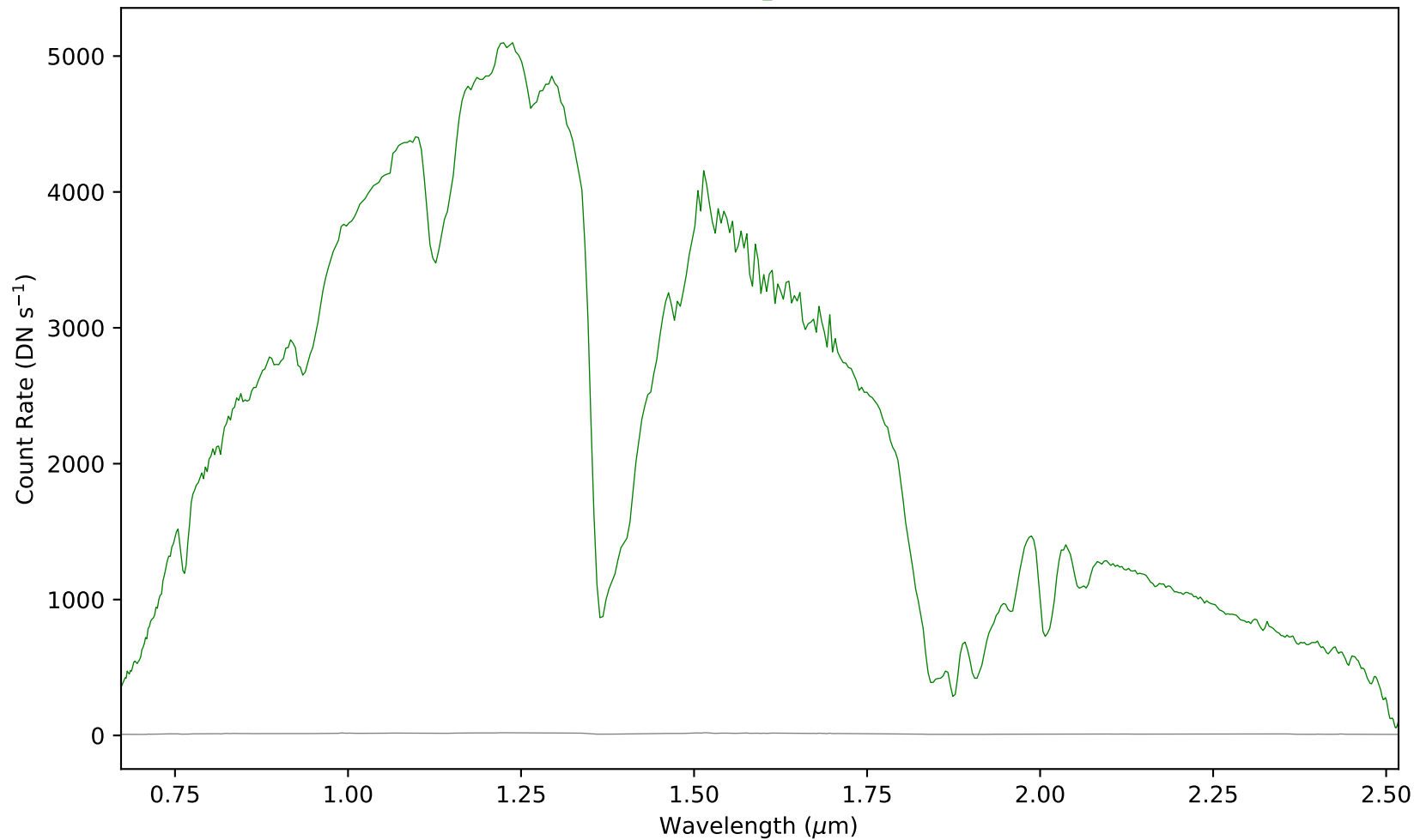
combspec248-403.fits - Aperture 1
