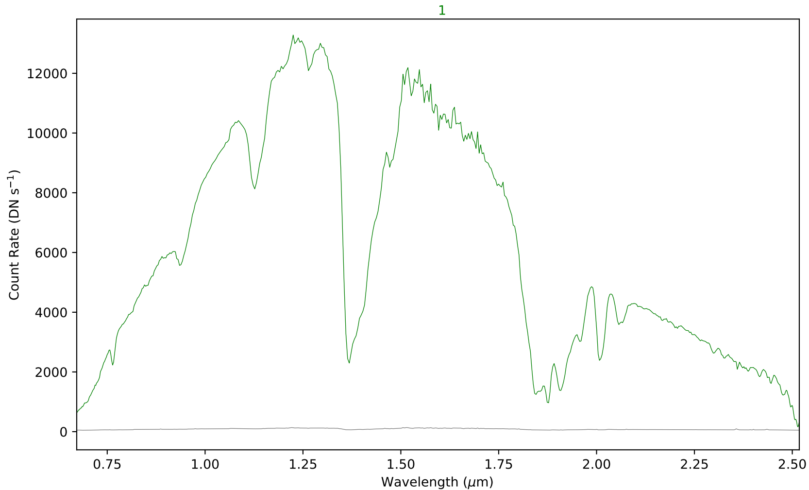
combspec258-413.fits - Aperture 1
