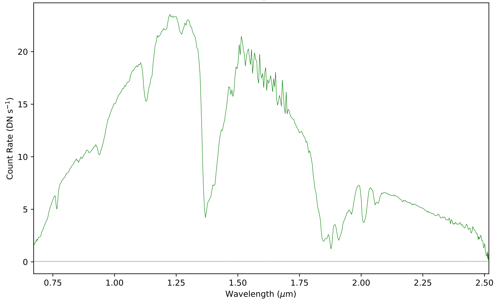
combspec268-277.fits - Aperture 1
