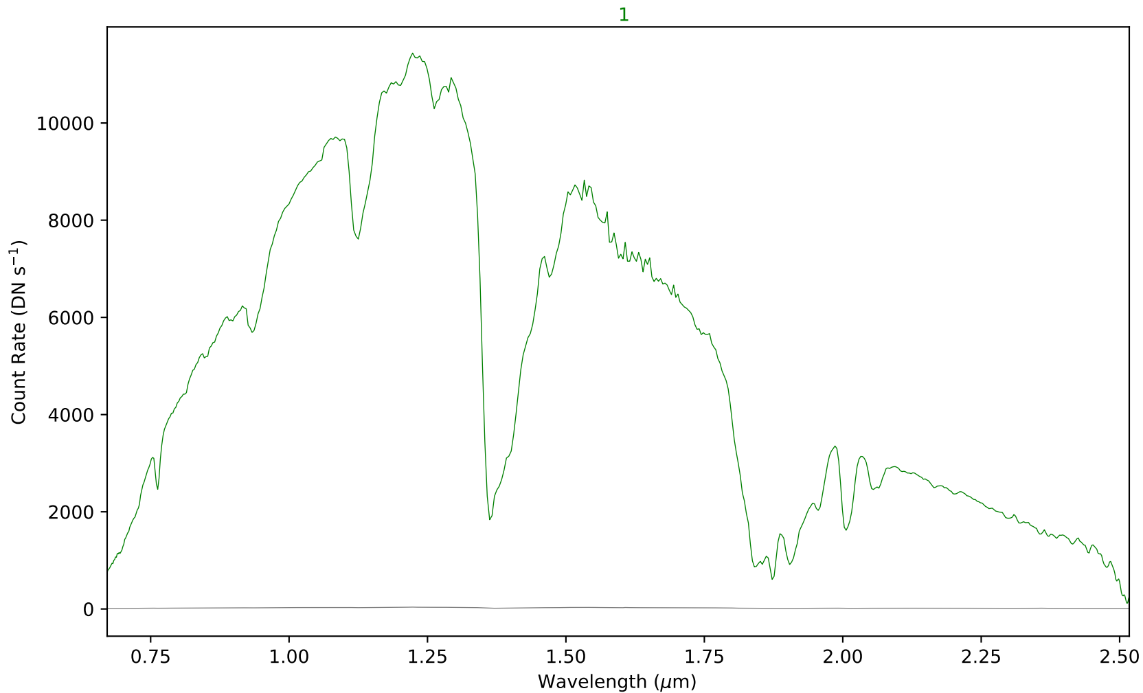
combspec29-159.fits - Aperture 1
