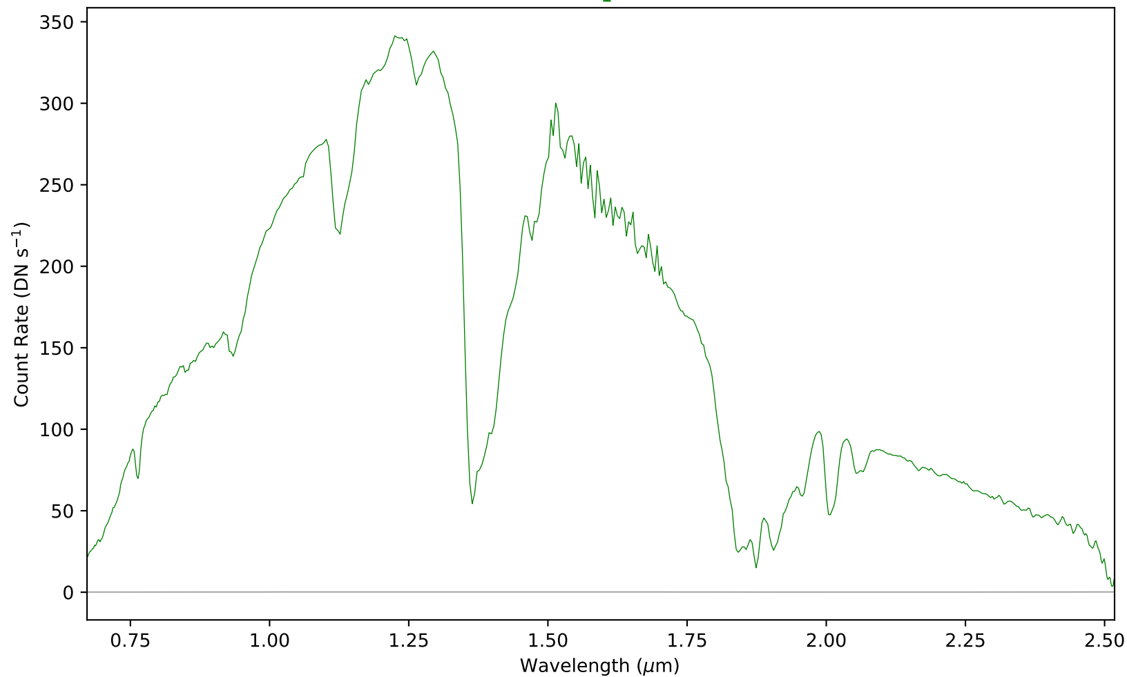
combspec308-313.fits - Aperture 1
