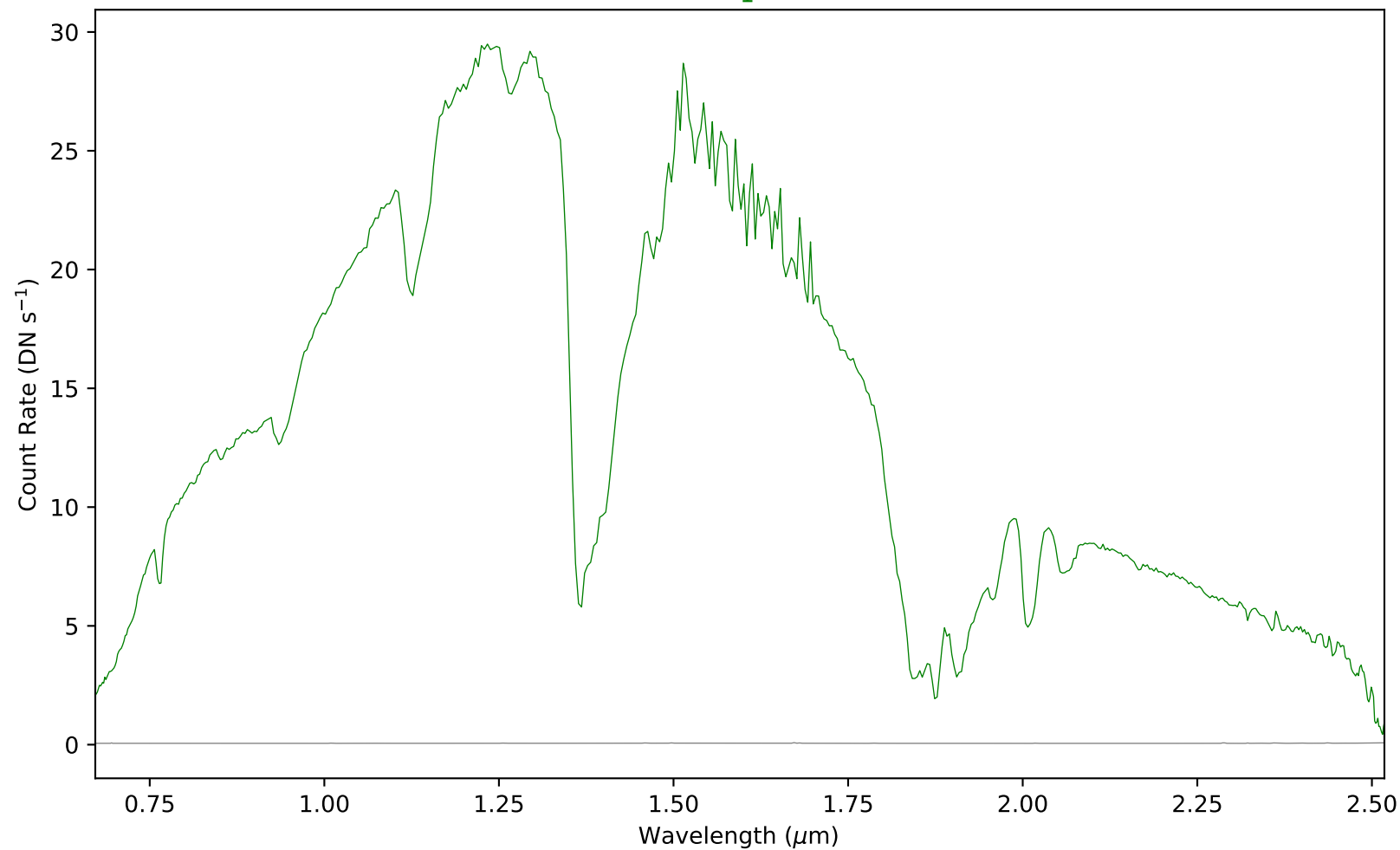
combspec326-341.fits - Aperture 1
