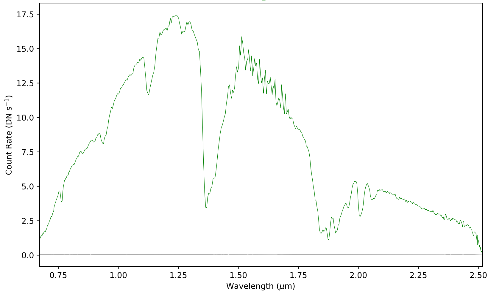
combspec342-349.fits - Aperture 1
