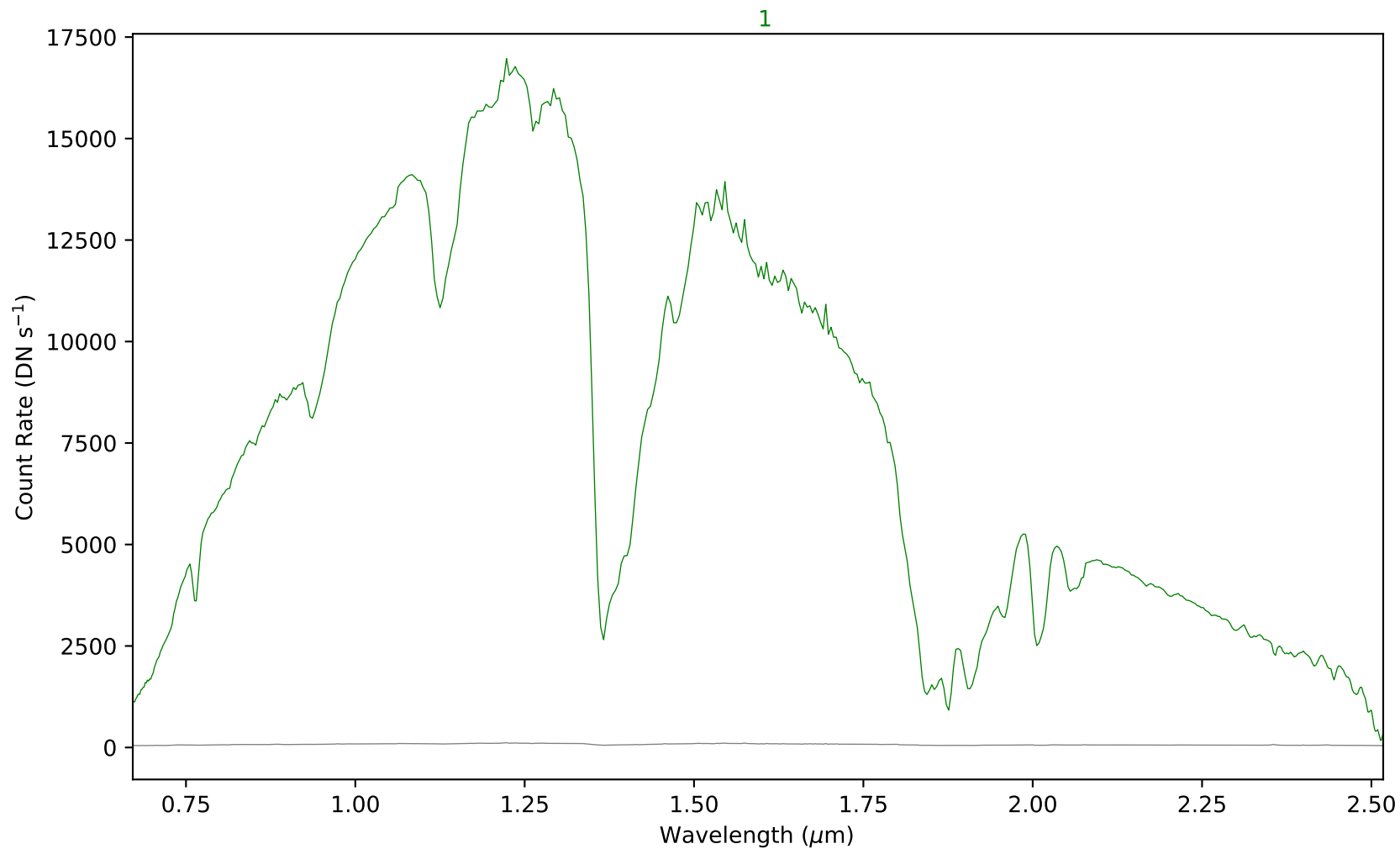
combspec39-233.fits - Aperture 1
