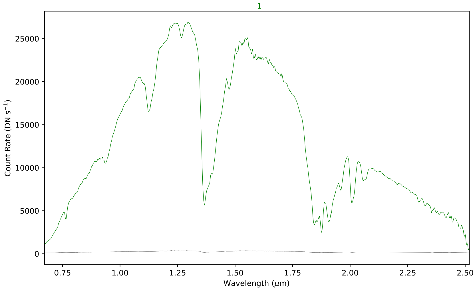
combspec414-451.fits - Aperture 1
