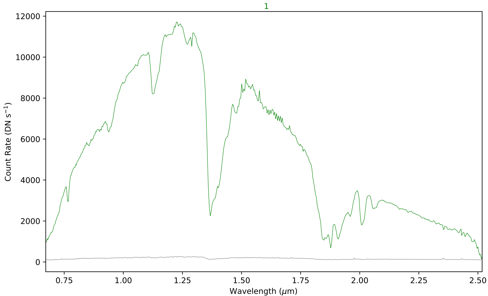
combspec452-461.fits - Aperture 1
