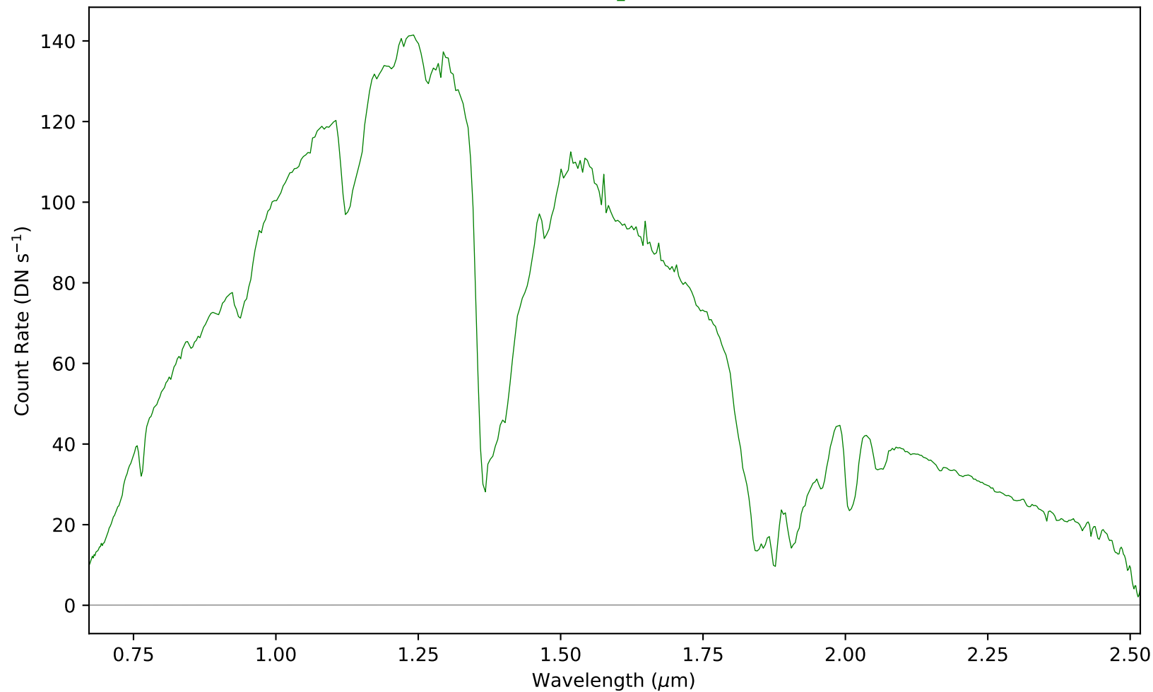
combspec482-491.fits - Aperture 1
