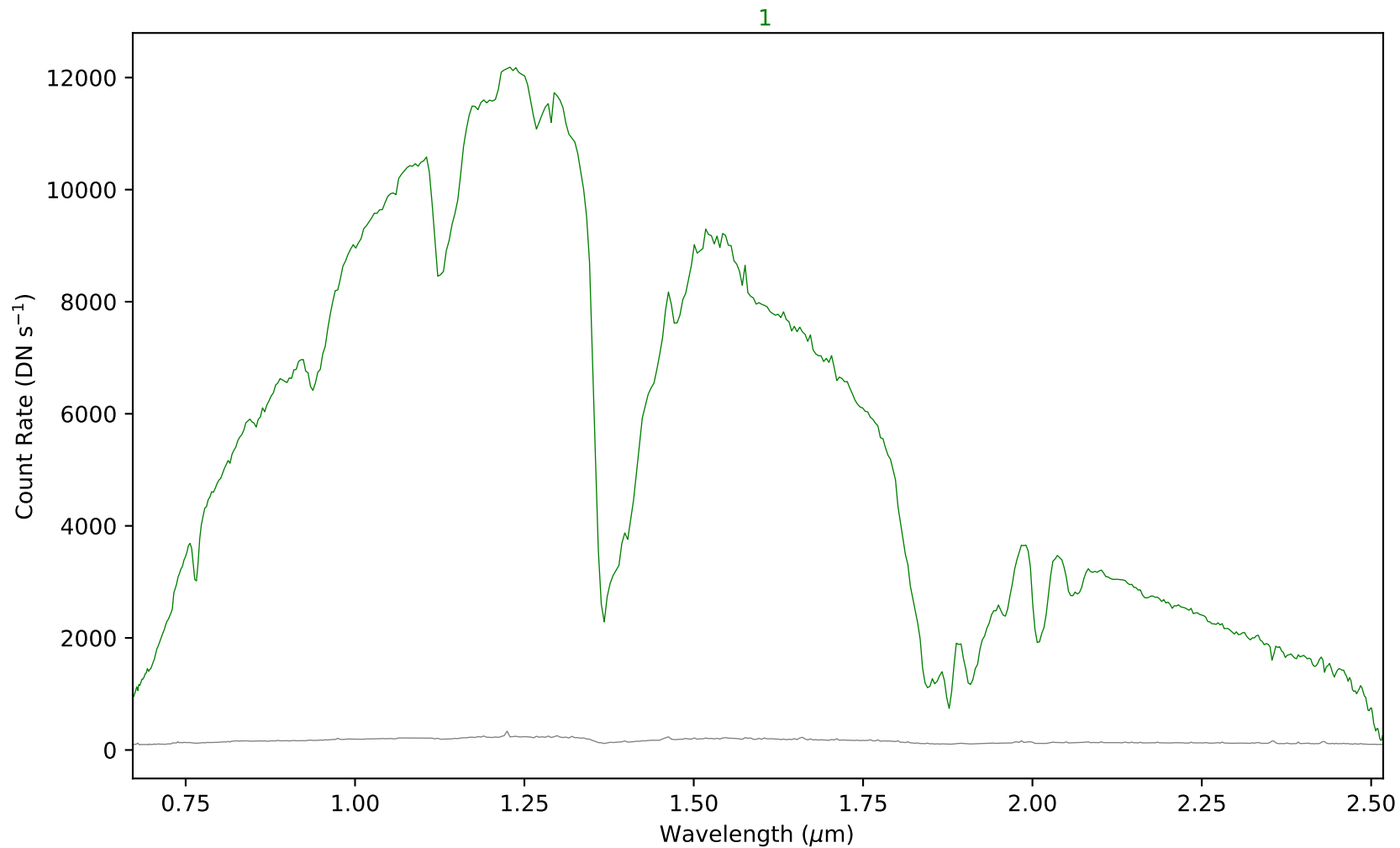
combspec502-511.fits - Aperture 1
