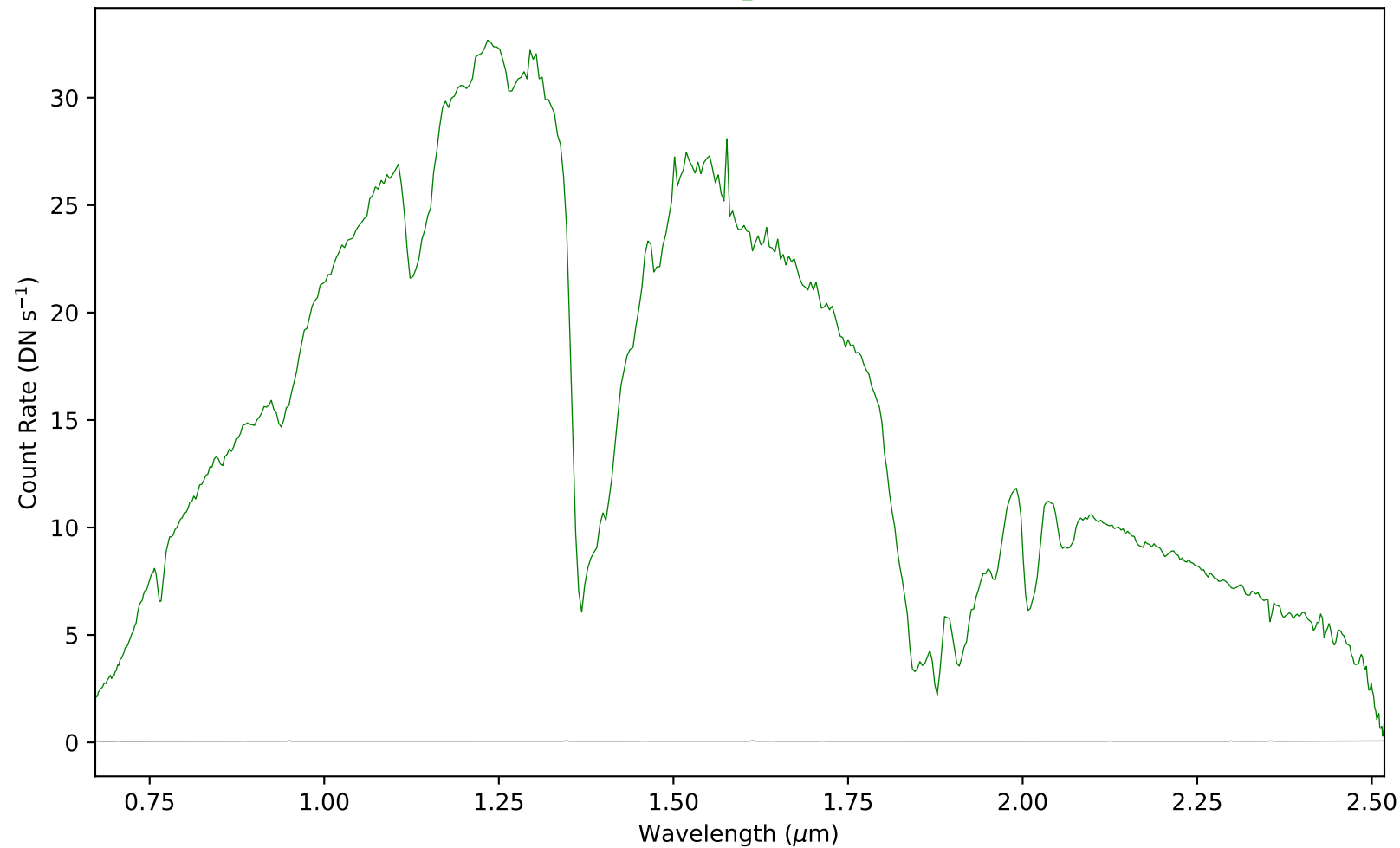
combspec532-539.fits - Aperture 1
