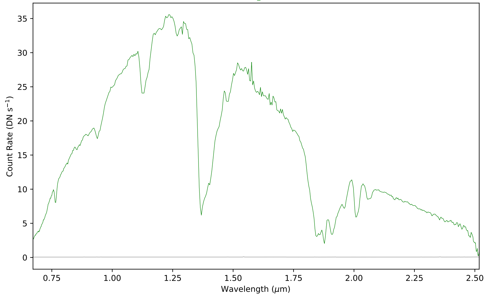
combspec540-547.fits - Aperture 1
