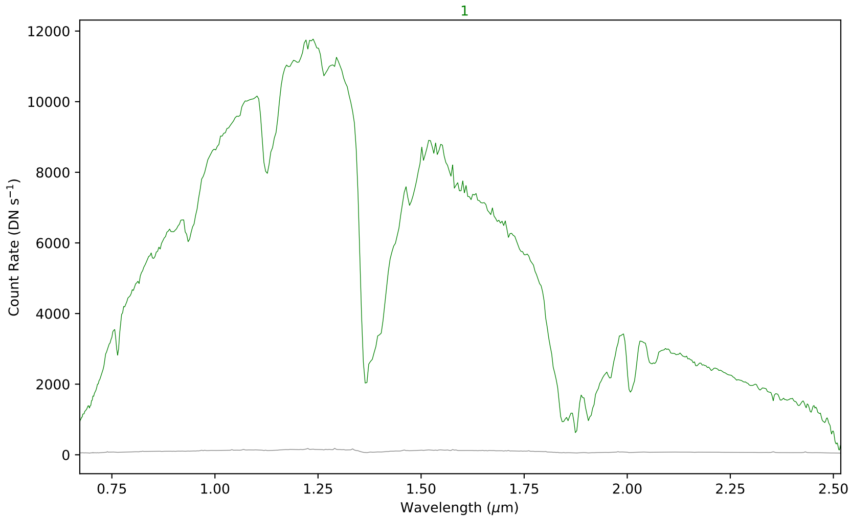
combspec558-567.fits - Aperture 1
