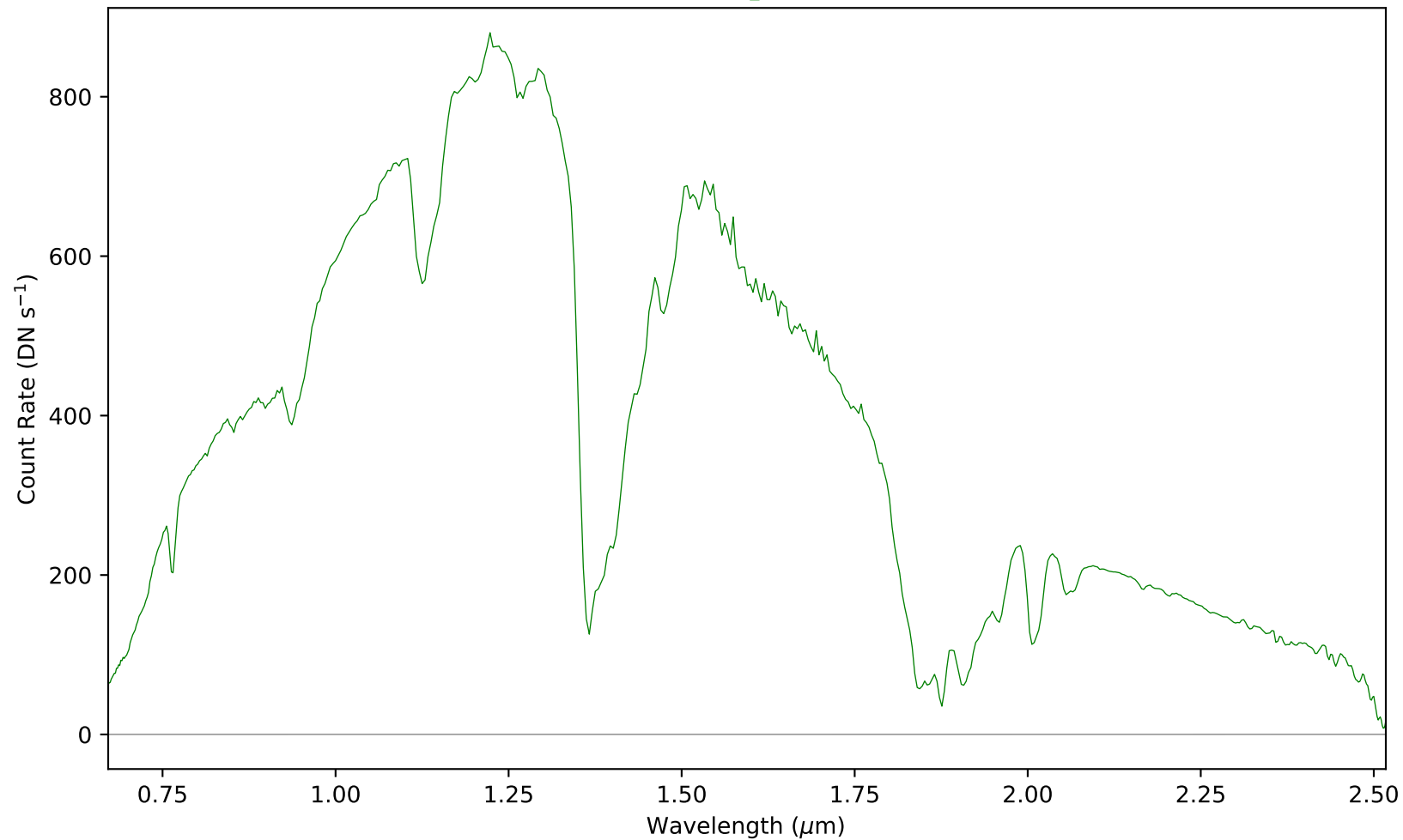
combspec61-74.fits - Aperture 1
