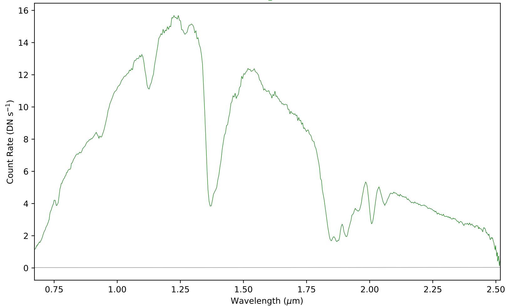
combspec167-266.fits - Aperture 1
