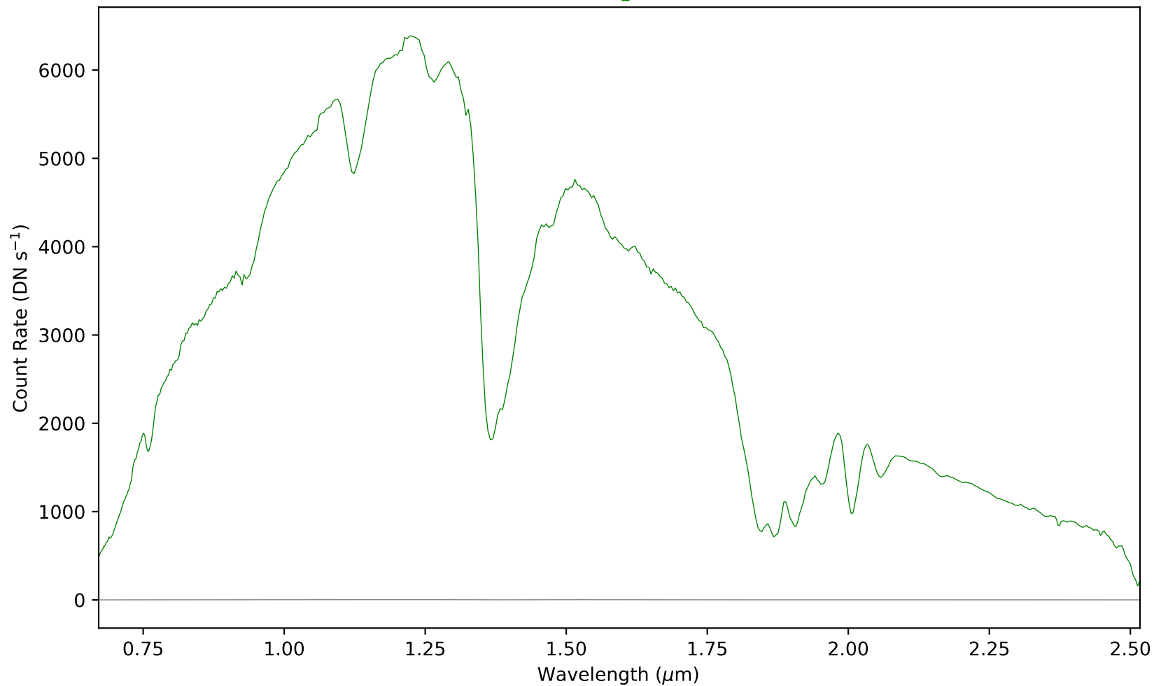
combspec191-306.fits - Aperture 1
