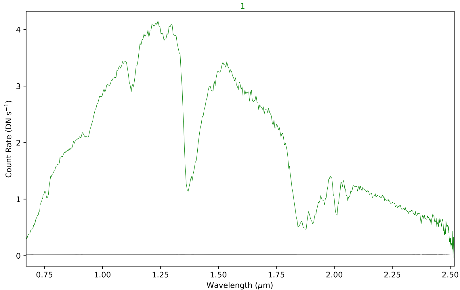
combspec203-296.fits - Aperture 1
