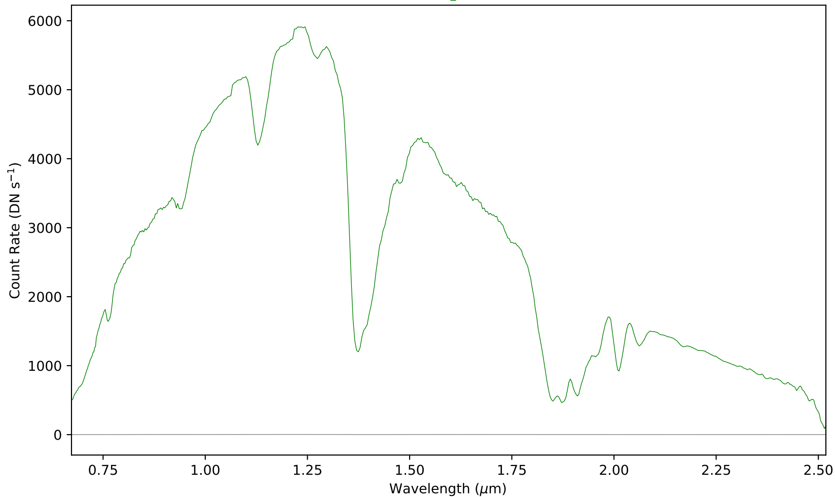
combspec23-140.fits - Aperture 1
