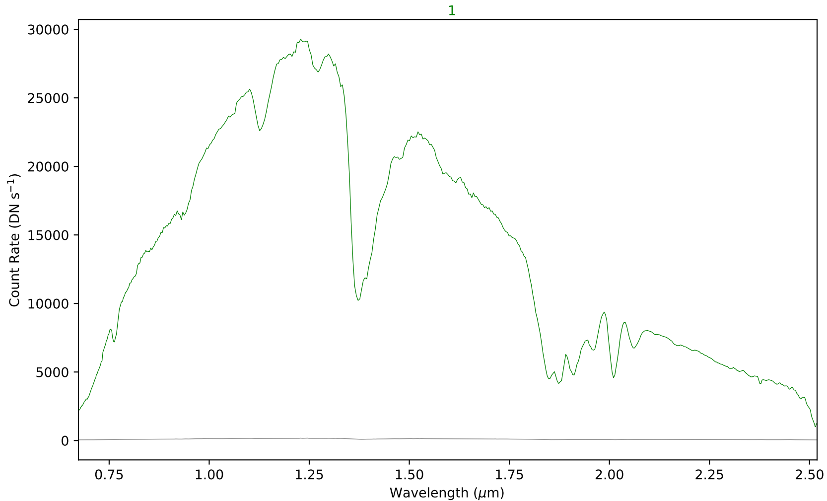
combspec323-368.fits - Aperture 1
