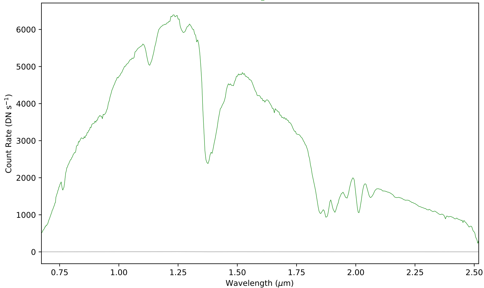
combspec379-414.fits - Aperture 1
