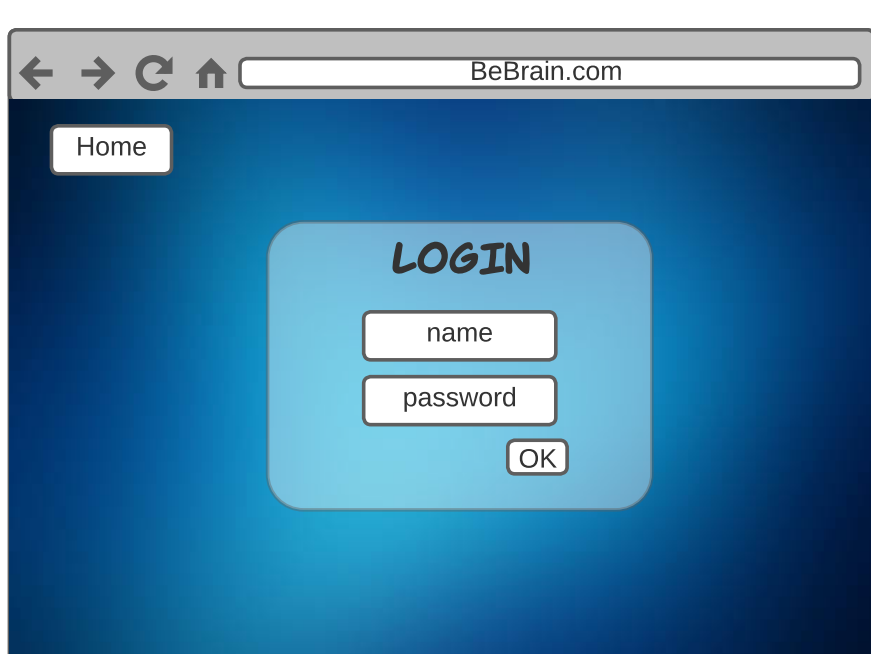
Login Screen
