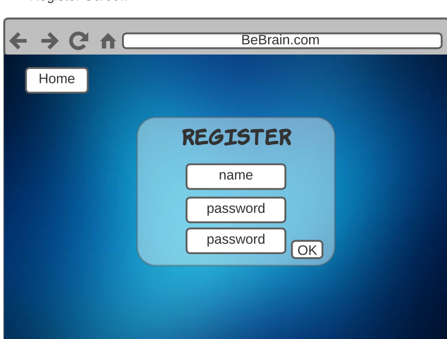
Register Screen
