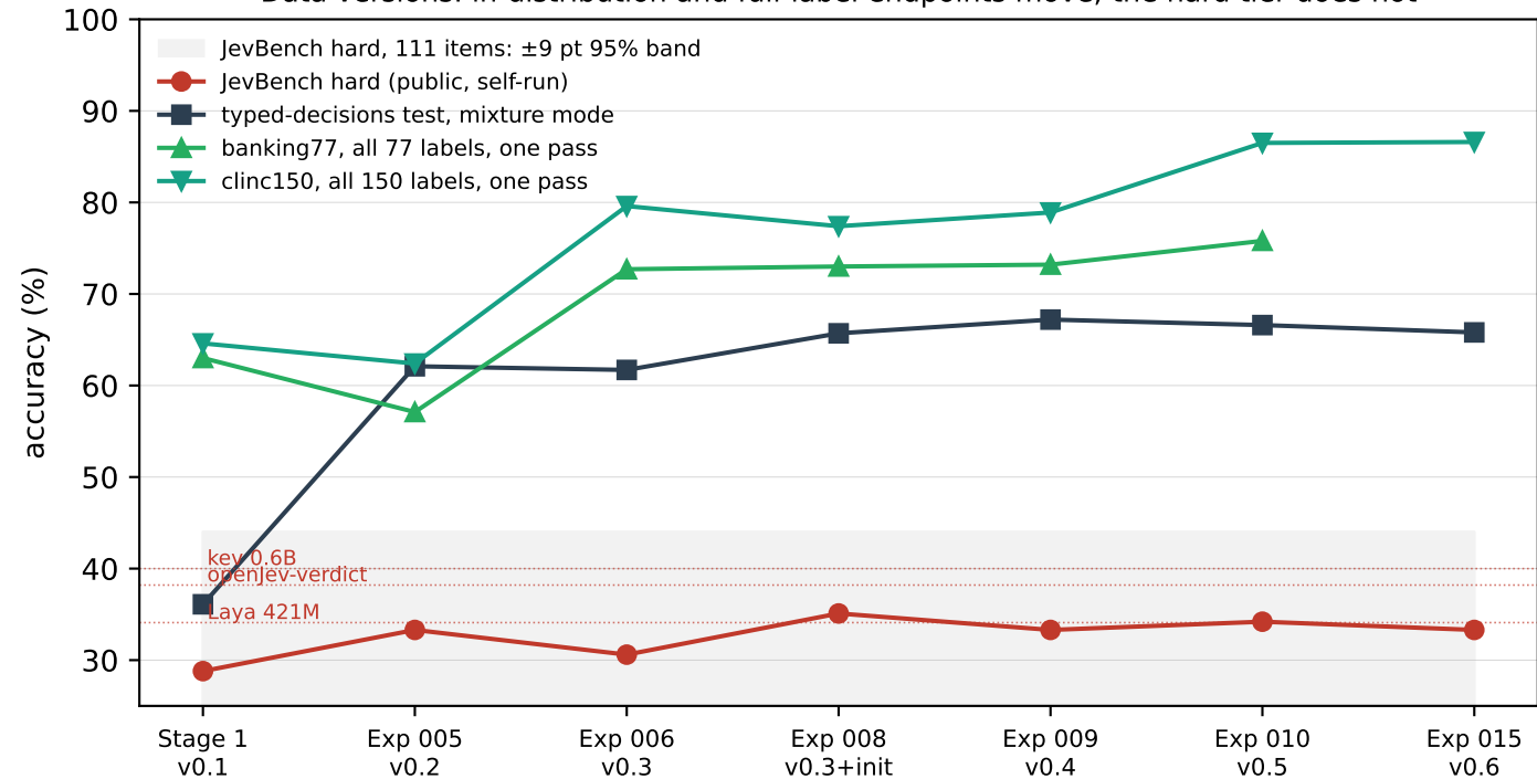
Data versions: in-distribution and full-label endpoints move; the hard tier does not
