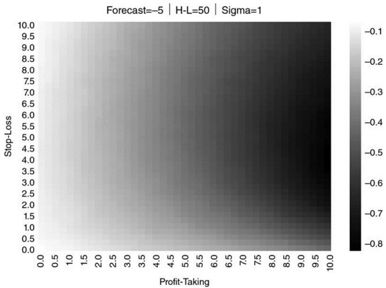
FIGURE 13.19 Heat-map for \{E_0[P_{i,T_i}], \tau, \sigma\} = \{-5, 50, 1\}
