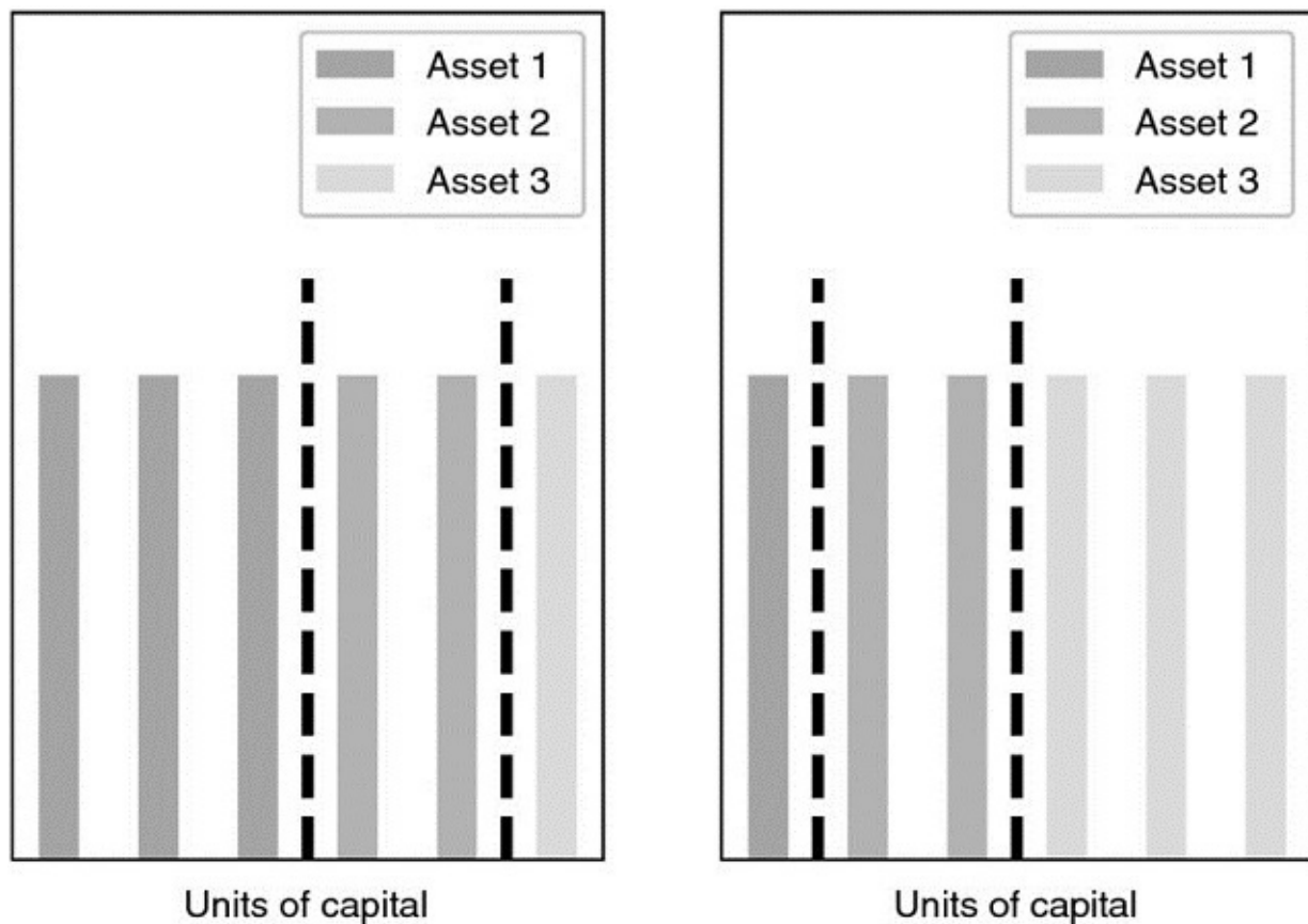
FIGURE 21.1 Partitions (1, 2, 3) and (3, 2, 1) must be treated as different
