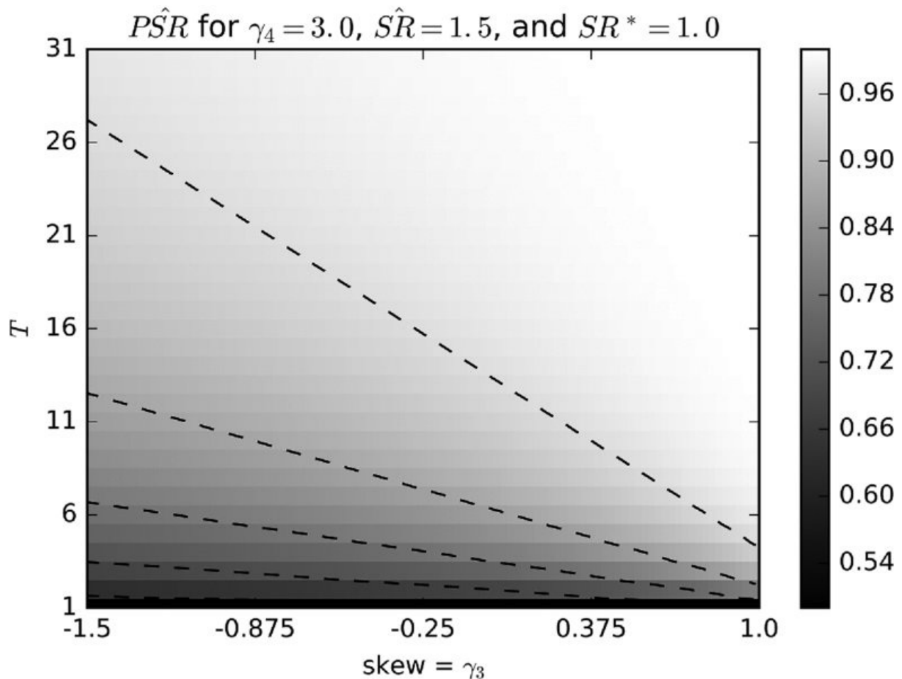
FIGURE 14.2 PSR as a function of skewness and sample length
