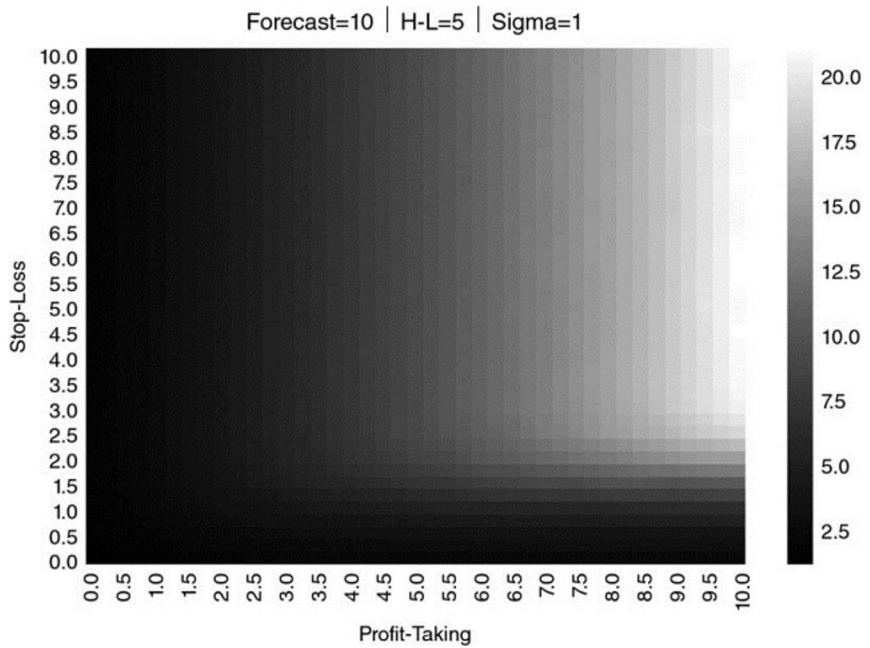
FIGURE 13.11 Heat-map for \{E_0[P_{i,T_i}], \tau, \sigma\} = \{10, 5, 1\}
