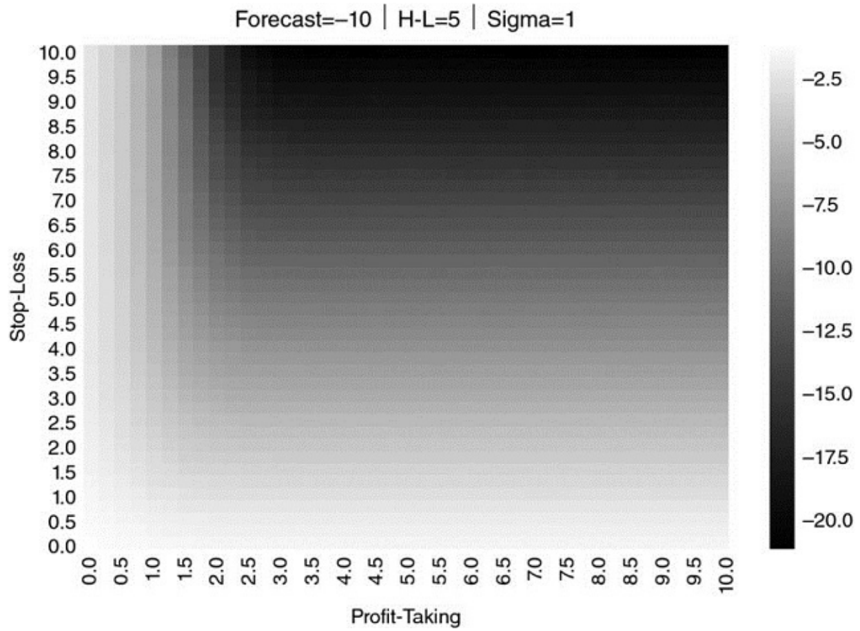
FIGURE 13.21 Heat-map for \{E_0[P_{i,T_i}], \tau, \sigma\} = \{-10, 5, 1\}
