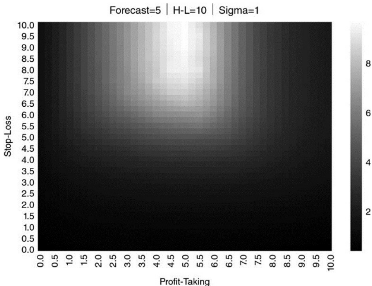
FIGURE 13.7 Heat-map for \{E_0[P_{i,T_i}], \tau, \sigma\} = \{5, 10, 1\}
