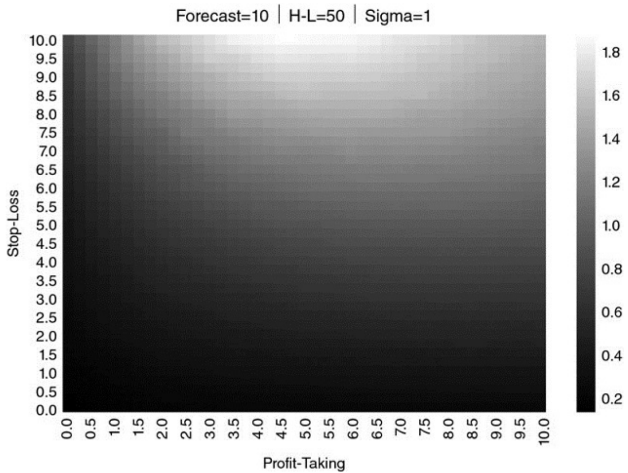
FIGURE 13.14 Heat-map for \{E_0[P_{i,T_i}], \tau, \sigma\} = \{10, 50, 1\}
