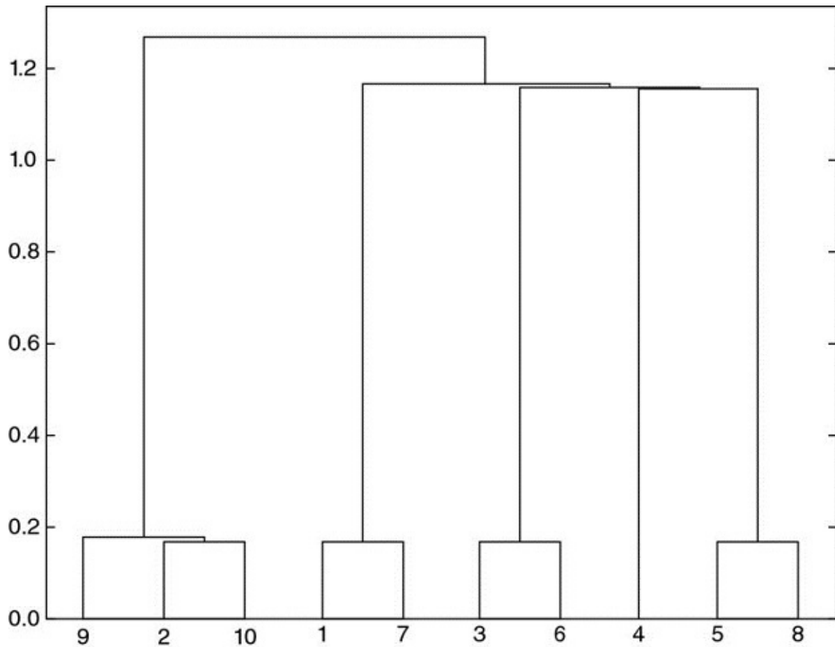
FIGURE 16.5 Dendrogram of cluster formation
