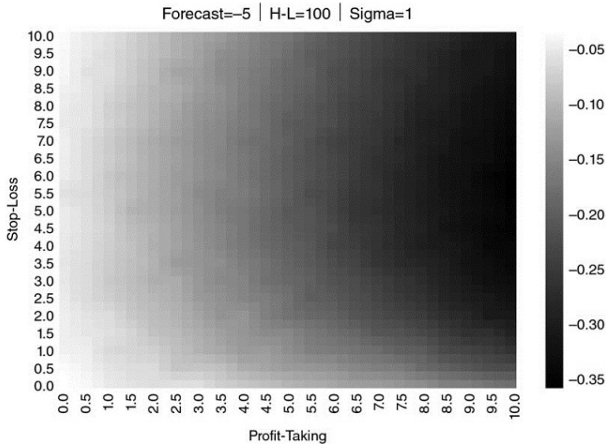
FIGURE 13.20 Heat-map for \{E_0[P_{i,T_i}], \tau, \sigma\} = \{-5, 100, 1\}
