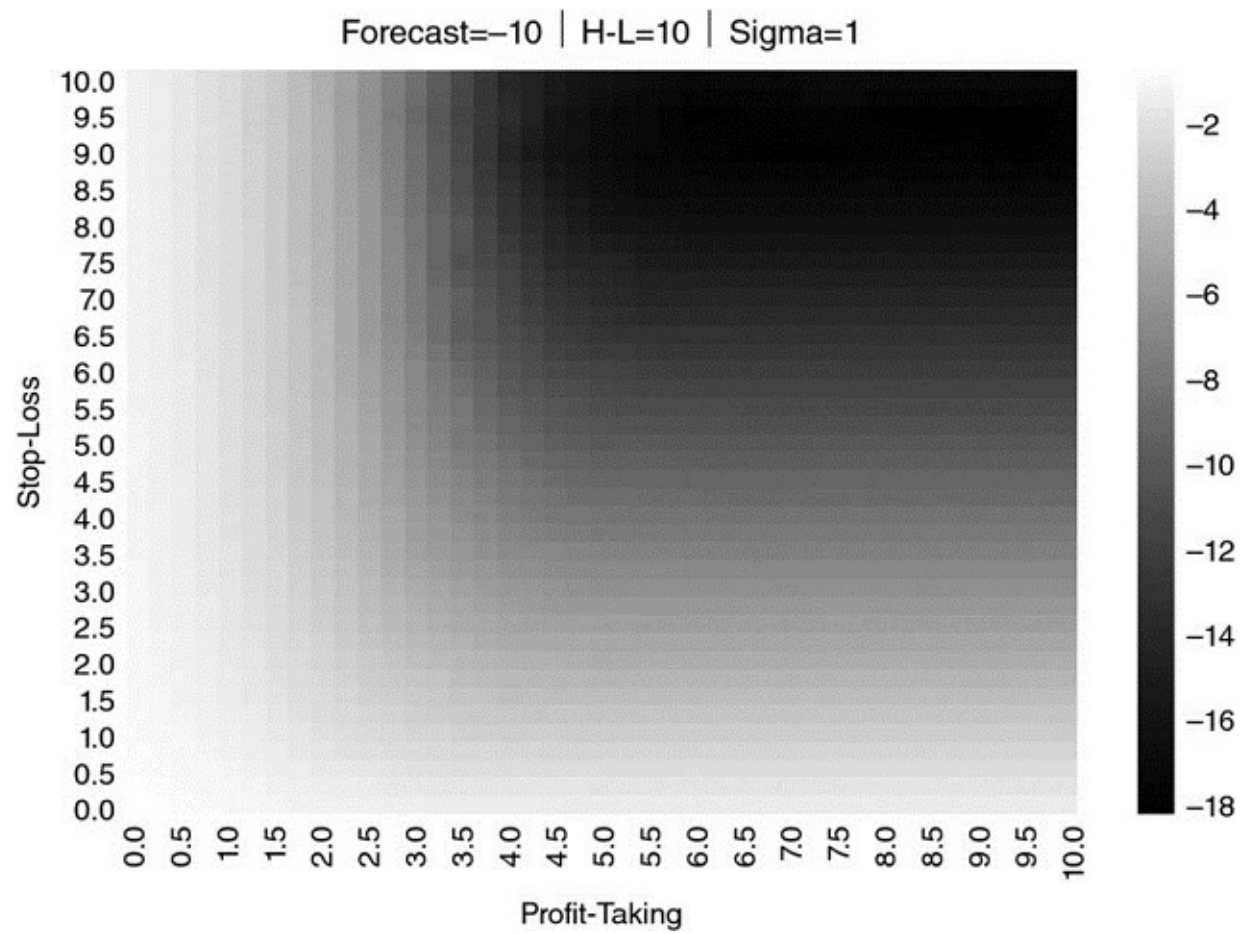
FIGURE 13.22 Heat-map for \{E_0[P_{i,T_i}], \tau, \sigma\} = \{-10, 10, 1\}
