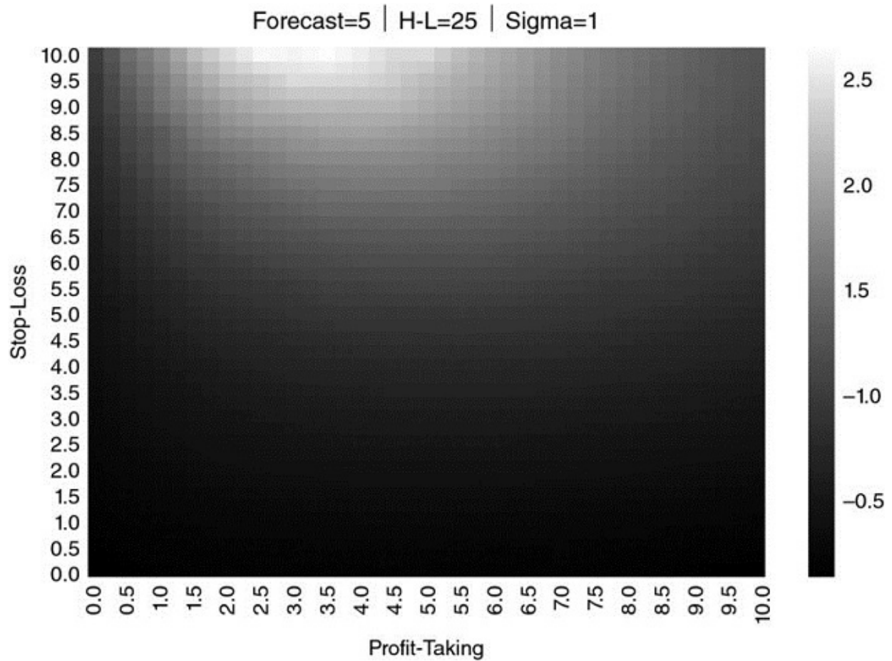
FIGURE 13.8 Heat-map for \{E_0[P_{i,T_i}], \tau, \sigma\} = \{5, 25, 1\}
