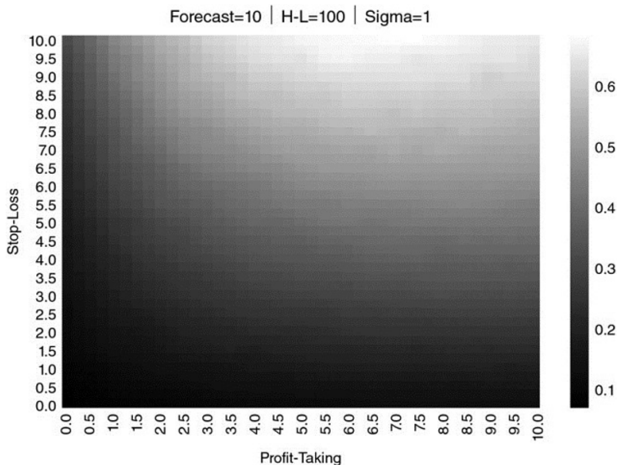
FIGURE 13.15 Heat-map for \{E_0[P_{i,T_i}], \tau, \sigma\} = \{10, 100, 1\}
