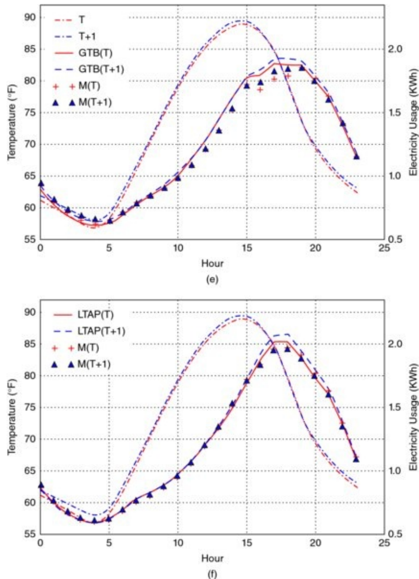
FIGURE 22.6 Gradient tree boosting (GBT) appears to follow recent usage too closely and therefore not able to predict the baseline usage as well as the newly develop method named LTAP. (a) GBT on Control group. (b) LTAP on Control group. (c) GBT on Passive group. (d) LTAP on Passive group. (e) GBT on Active group. (f) LTAP on Active group
