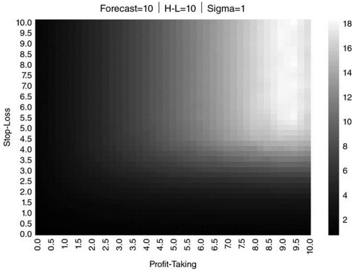
FIGURE 13.12 Heat-map for \{E_0[P_{i,T_i}], \tau, \sigma\} = \{10, 10, 1\}
