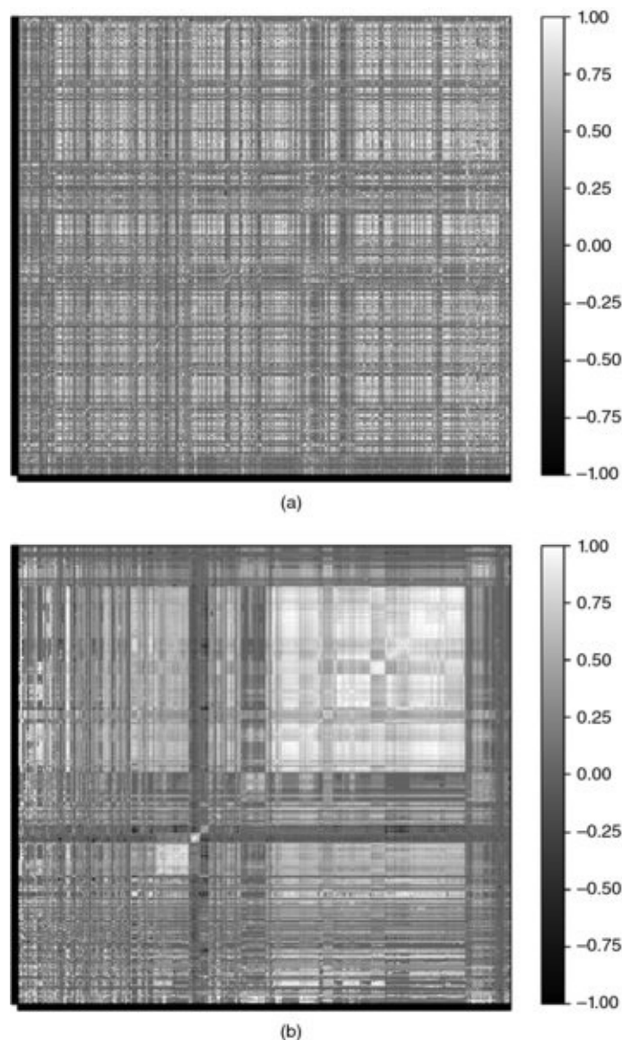
FIGURE 16.8 Correlation matrix before and after clustering
