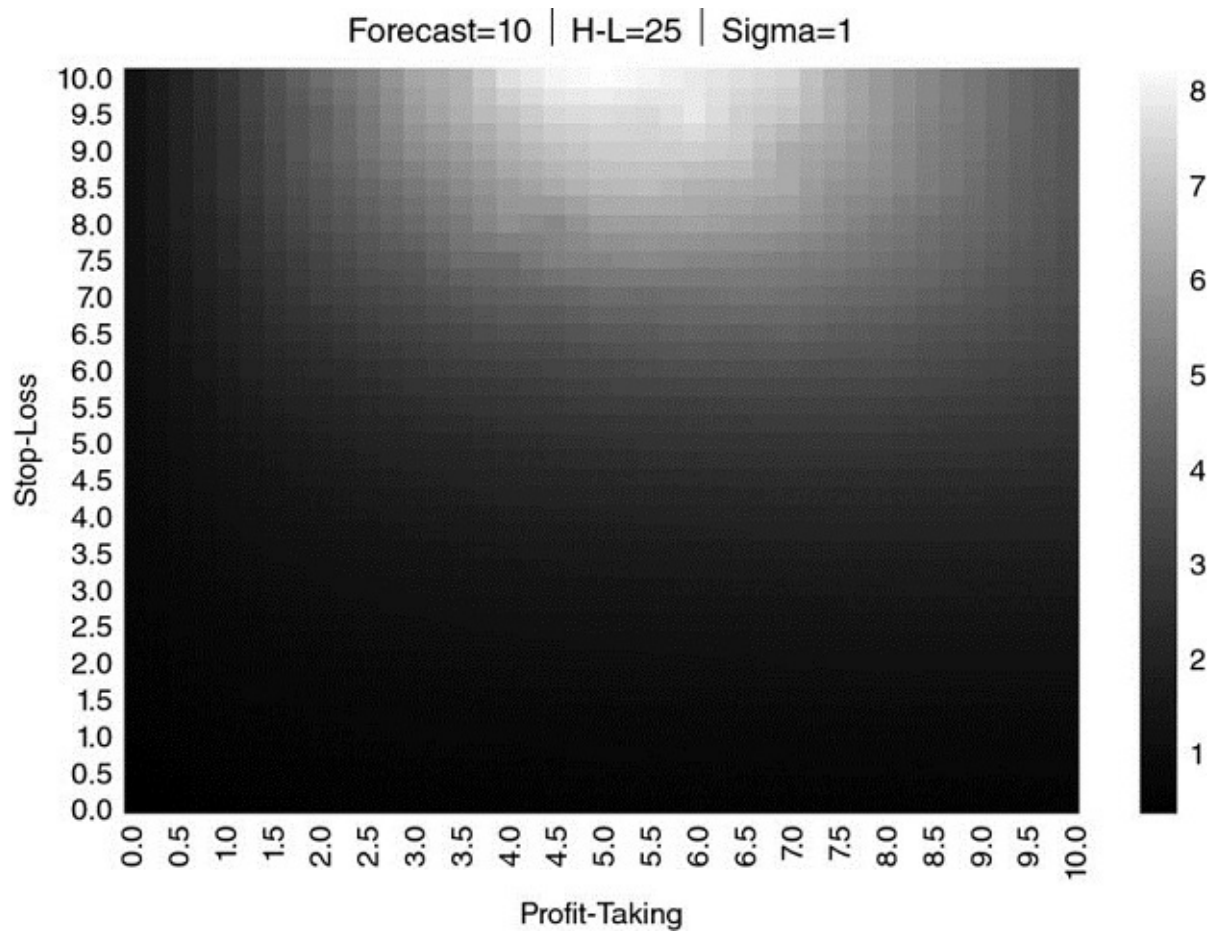
FIGURE 13.13 Heat-map for \{E_0[P_{i,T_i}], \tau, \sigma\} = \{10, 25, 1\}
