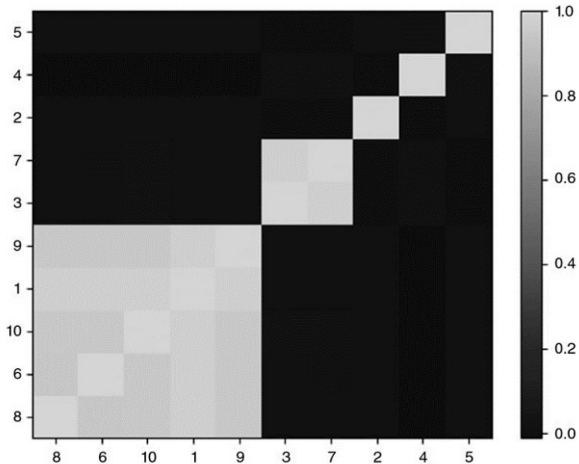
FIGURE 16.6 Clustered covariance matrix
