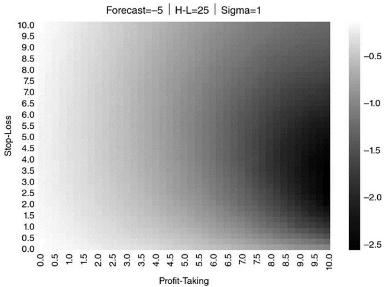
FIGURE 13.18 Heat-map for \{E_0[P_{i,T_i}], \tau, \sigma\} = \{-5, 25, 1\}
