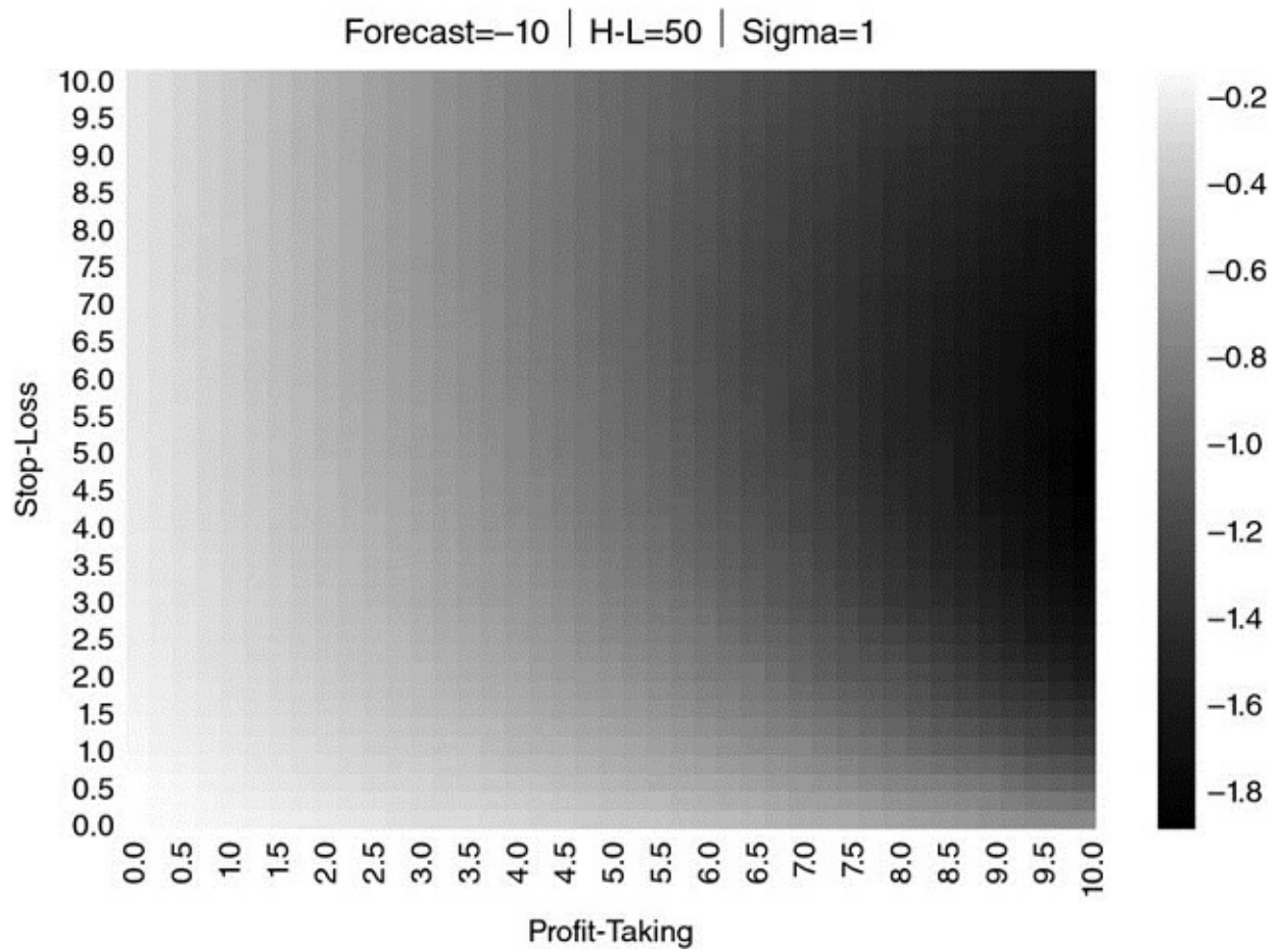
FIGURE 13.24 Heat-map for \{E_0[P_{i,T_i}], \tau, \sigma\} = \{-10, 50, 1\}
