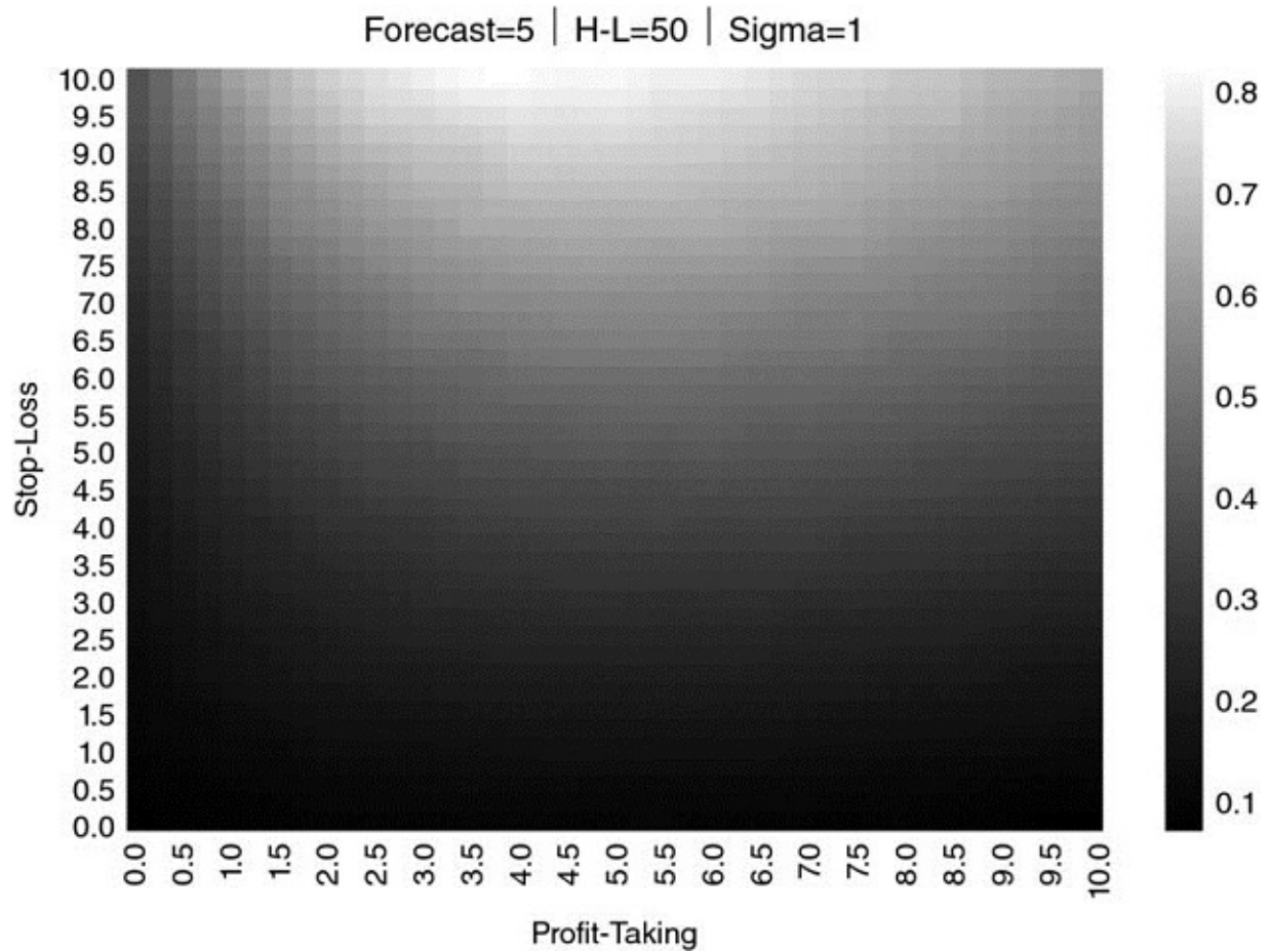
FIGURE 13.9 Heat-map for \{E_0[P_{i,T_i}], \tau, \sigma\} = \{5, 50, 1\}
