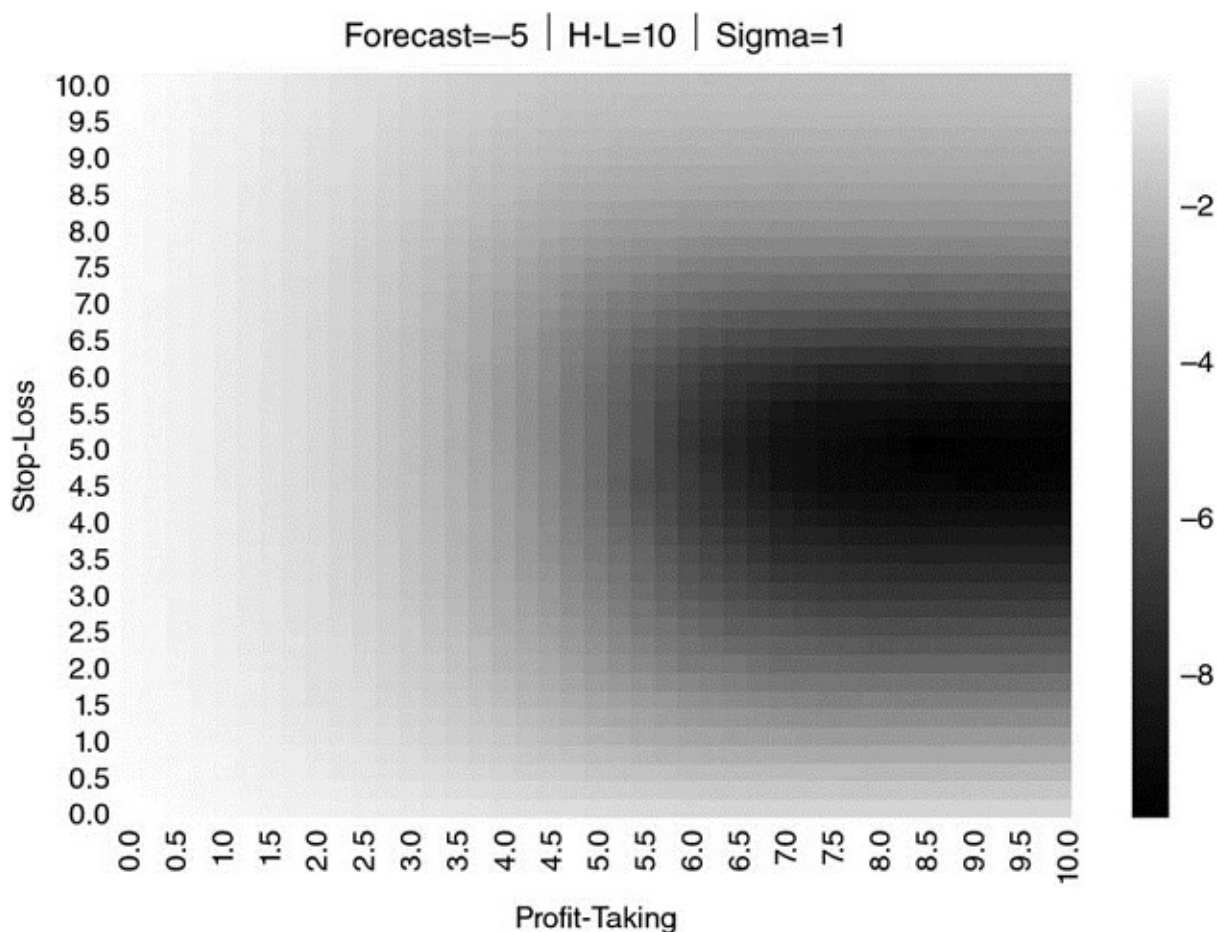
FIGURE 13.17 Heat-map for \{E_0[P_{i,T_i}], \tau, \sigma\} = \{-5, 10, 1\}
