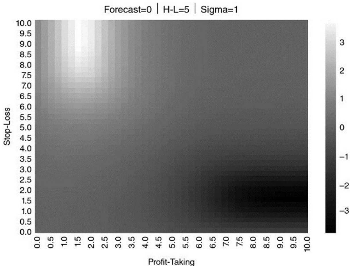
FIGURE 13.1 Heat-map for \{E_0[P_{i,T_i}], \tau, \sigma\} = \{0, 5, 1\}
