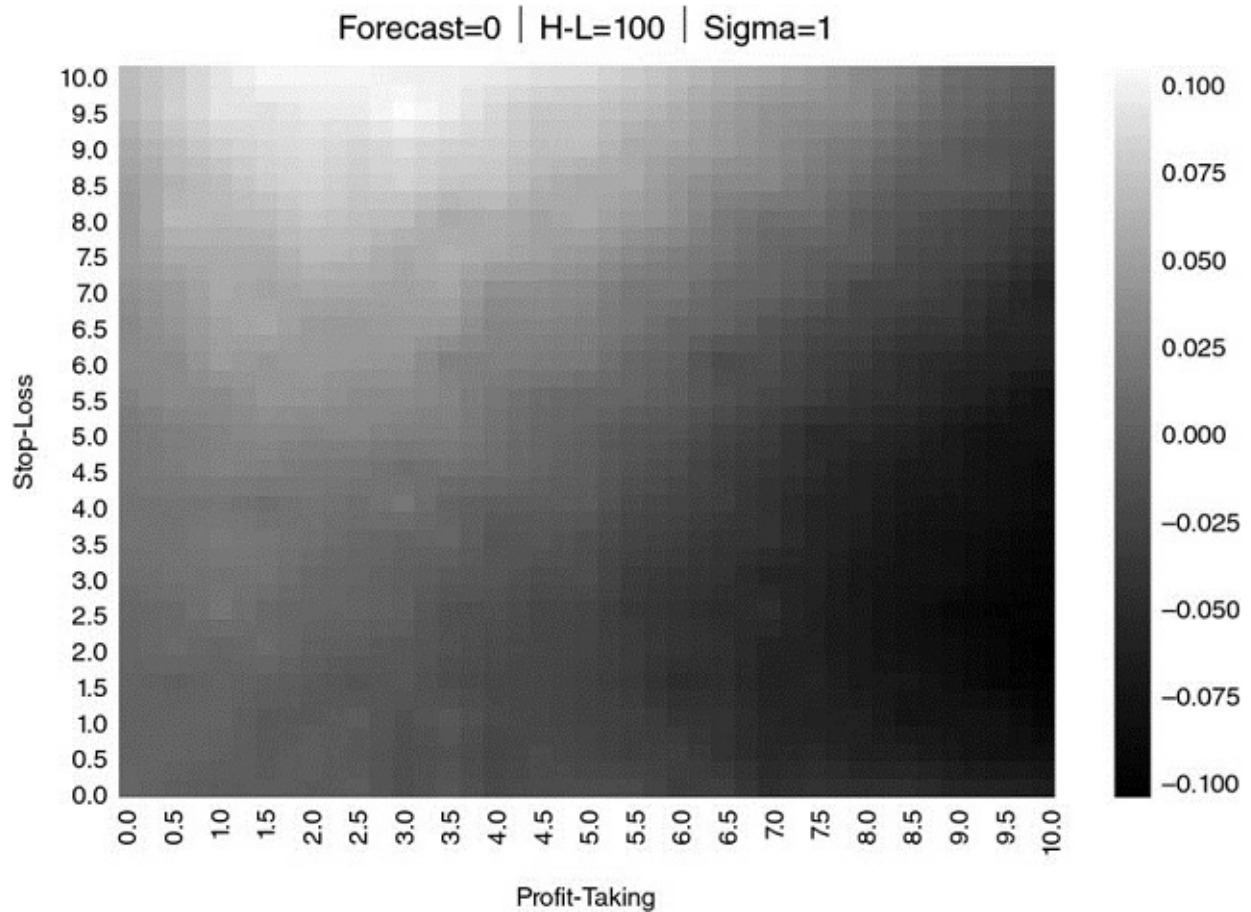
FIGURE 13.5 Heat-map for \{E_0[P_{i,T_i}], \tau, \sigma\} = \{0, 100, 1\}
