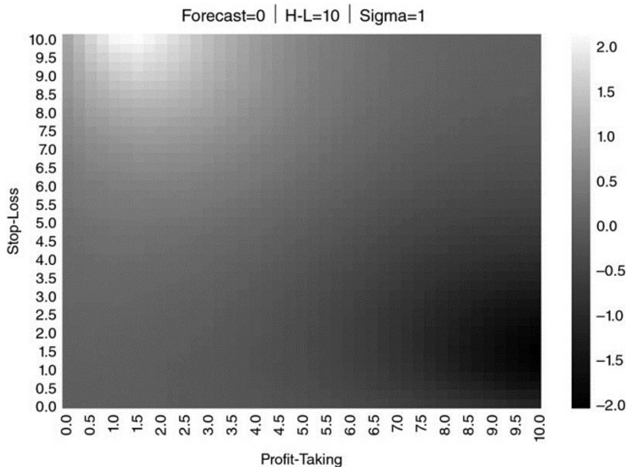
FIGURE 13.2 Heat-map for \{E_0[P_{i,T_i}], \tau, \sigma\} = \{0, 10, 1\}
