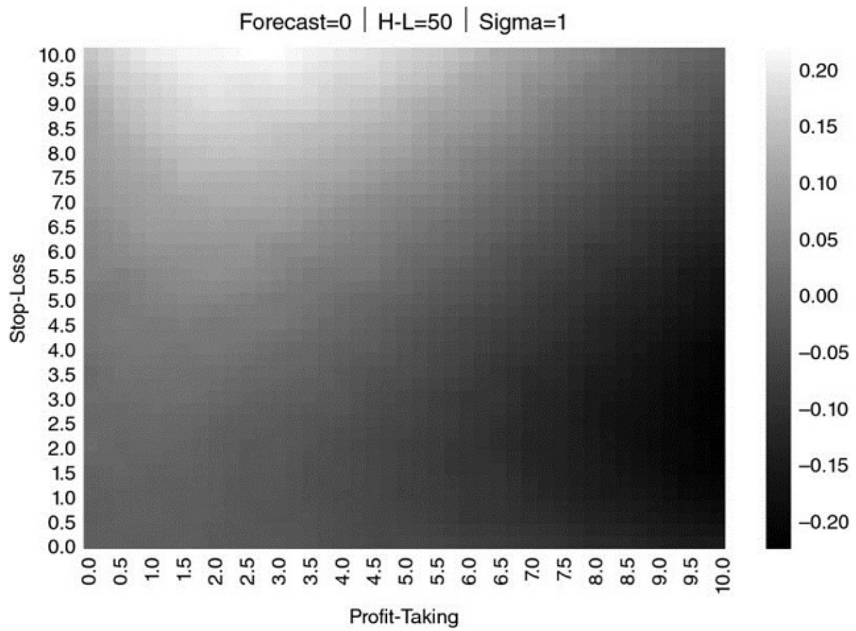
FIGURE 13.4 Heat-map for \{E_0[P_{i,T_i}], \tau, \sigma\} = \{0, 50, 1\}
