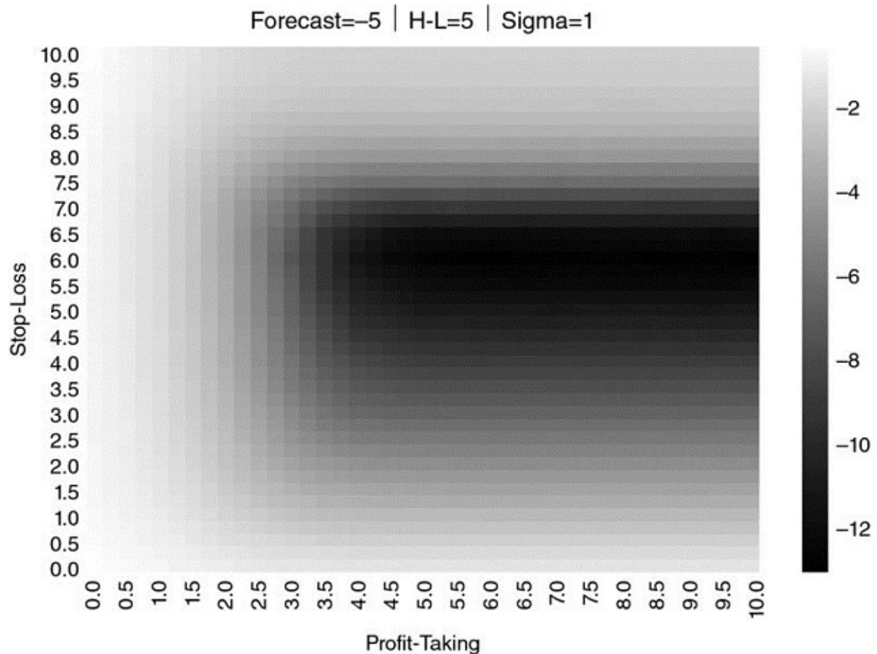
FIGURE 13.16 Heat-map for \{E_0[P_{i,T_i}], \tau, \sigma\} = \{-5, 5, 1\}
