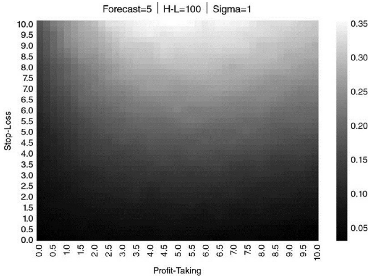
FIGURE 13.10 Heat-map for \{E_0[P_{i,T_i}], \tau, \sigma\} = \{5, 100, 1\}
