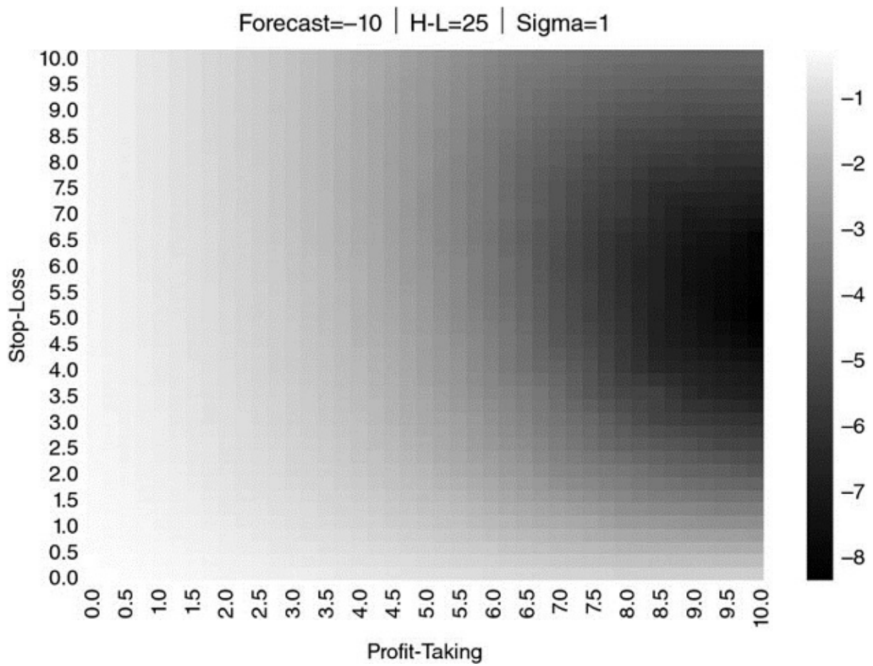
FIGURE 13.23 Heat-map for \{E_0[P_{i,T_i}], \tau, \sigma\} = \{-10, 25, 1\}
