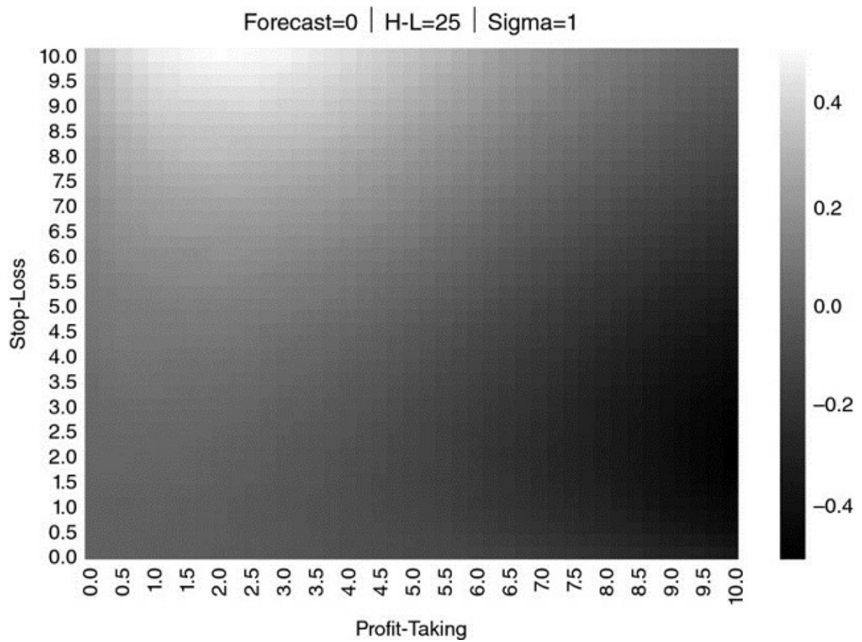
FIGURE 13.3 Heat-map for \{E_0[P_{i,T_i}], \tau, \sigma\} = \{0, 25, 1\}
