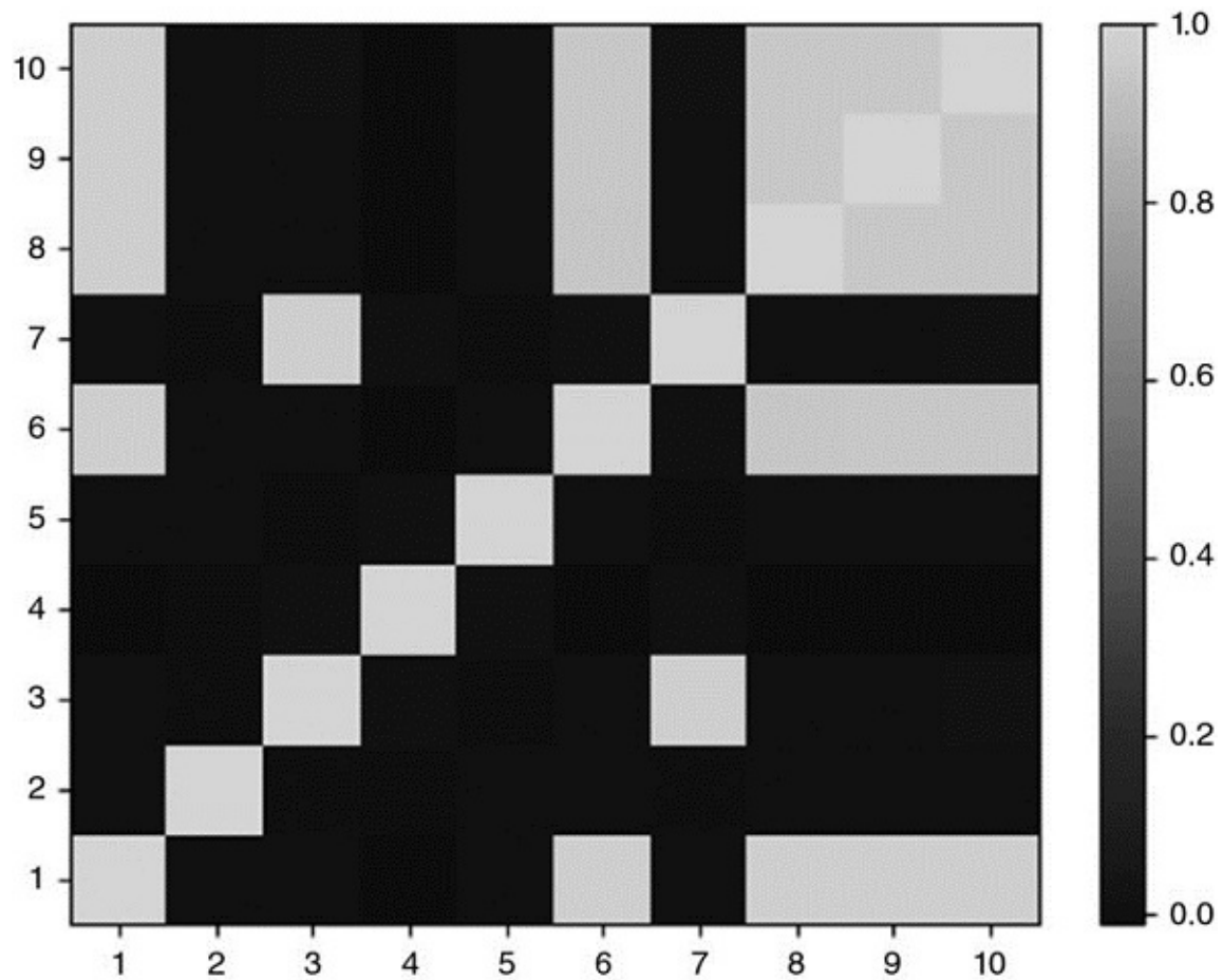
FIGURE 16.4 Heat-map of original covariance matrix
