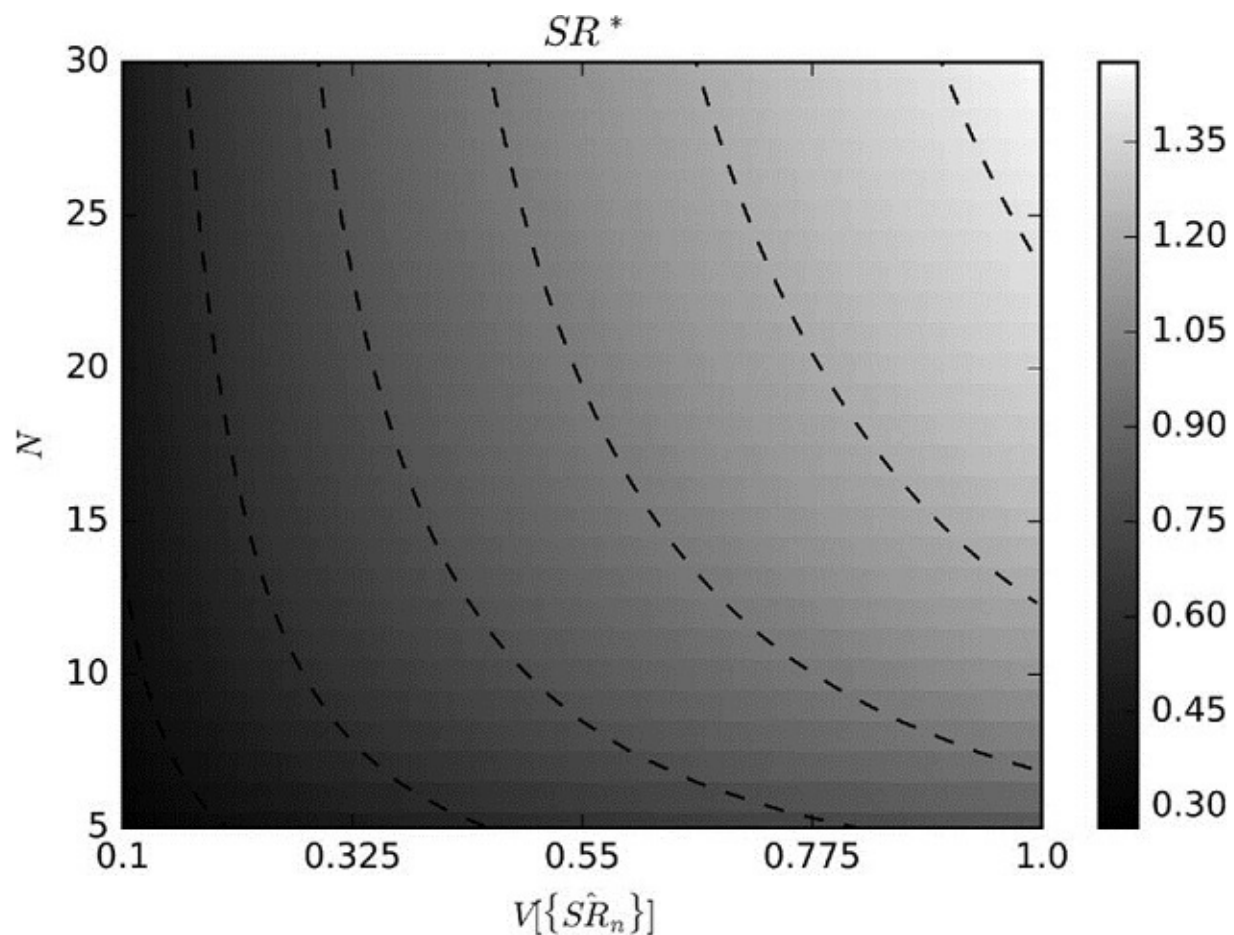
FIGURE 14.3 SR^* as a function of V[\{\widehat{SR}_n\}] and N
