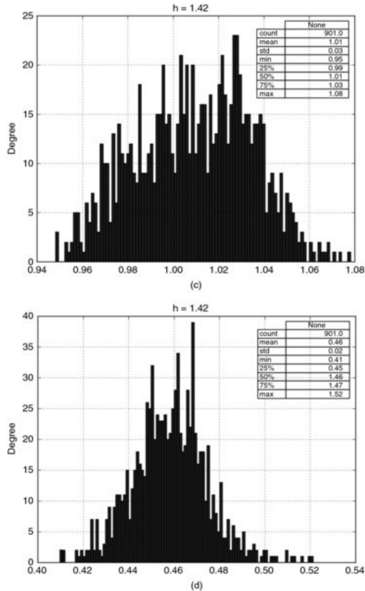
FIGURE 18.1 Distribution of entropy estimates under 10 (top), 7 (bottom), letter encodings, on messages of length 100 Distribution of entropy estimates under 5 (top), and 2 (bottom) letter encodings, on messages of length 100
