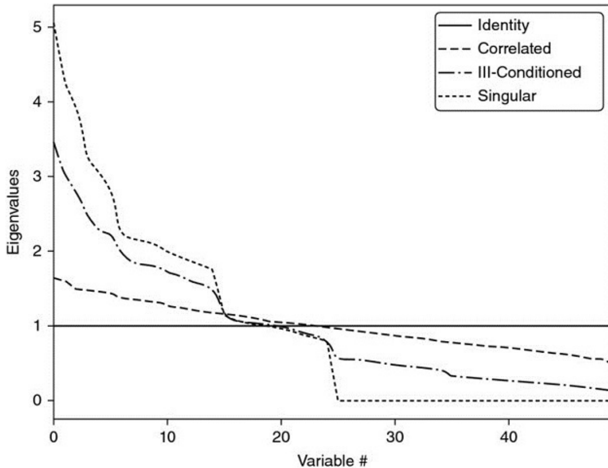
FIGURE 16.1 Visualization of Markowitz's curse
