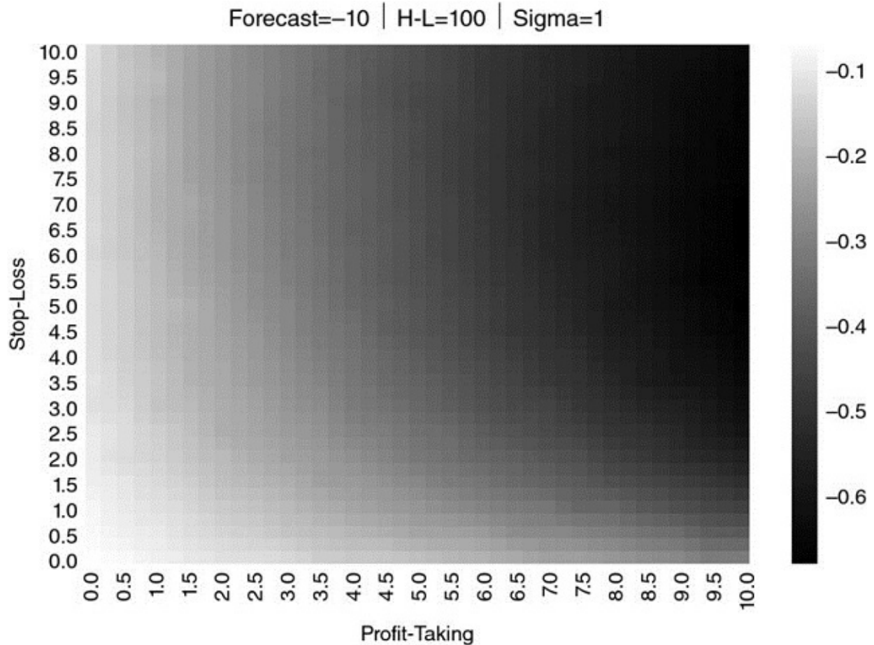
FIGURE 13.25 Heat-map for \{E_0[P_{i,T_i}], \tau, \sigma\} = \{-10, 100, 1\}
