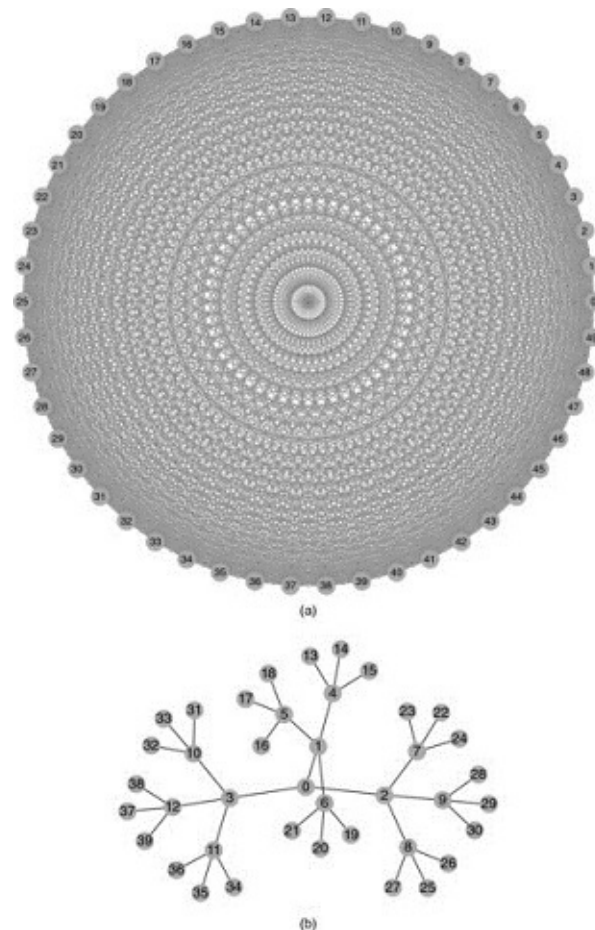
FIGURE 16.2 The complete-graph (top) and the tree-graph (bottom) structures. Correlation matrices can be represented as complete graphs, which lack the notion of hierarchy: Each investment is substitutable with another. In contrast, tree structures incorporate hierarchical relationships.
