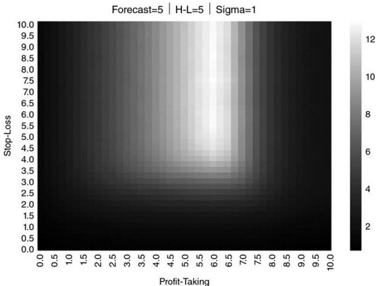
FIGURE 13.6 Heat-map for \{E_0[P_{i,T_i}], \tau, \sigma\} = \{5, 5, 1\}
