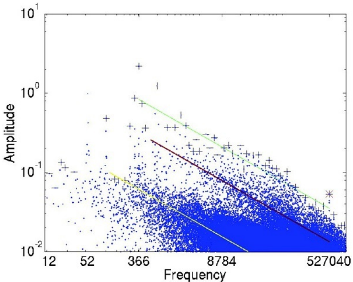
FIGURE 22.10 Fourier spectrum of trading prices of natural gas futures contracts in 2012. Non-uniform FFT identifies strong presence of activities happening once per day (frequency = 366), twice per day (frequency = 732), and once per minute (frequency = 527040 = 366 \times 24 \times 60 ).
