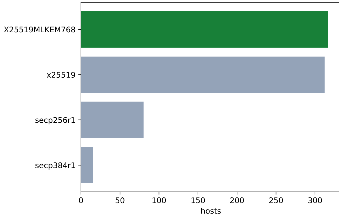
Negotiated key-exchange group (PQ-capable client)
