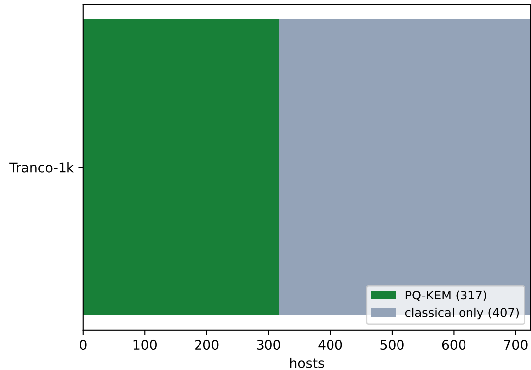
PQ-KEM negotiation when client advertises X25519MLKEM768 (rustls + rustls-post-quantum; 317/724 = 43.8%)
